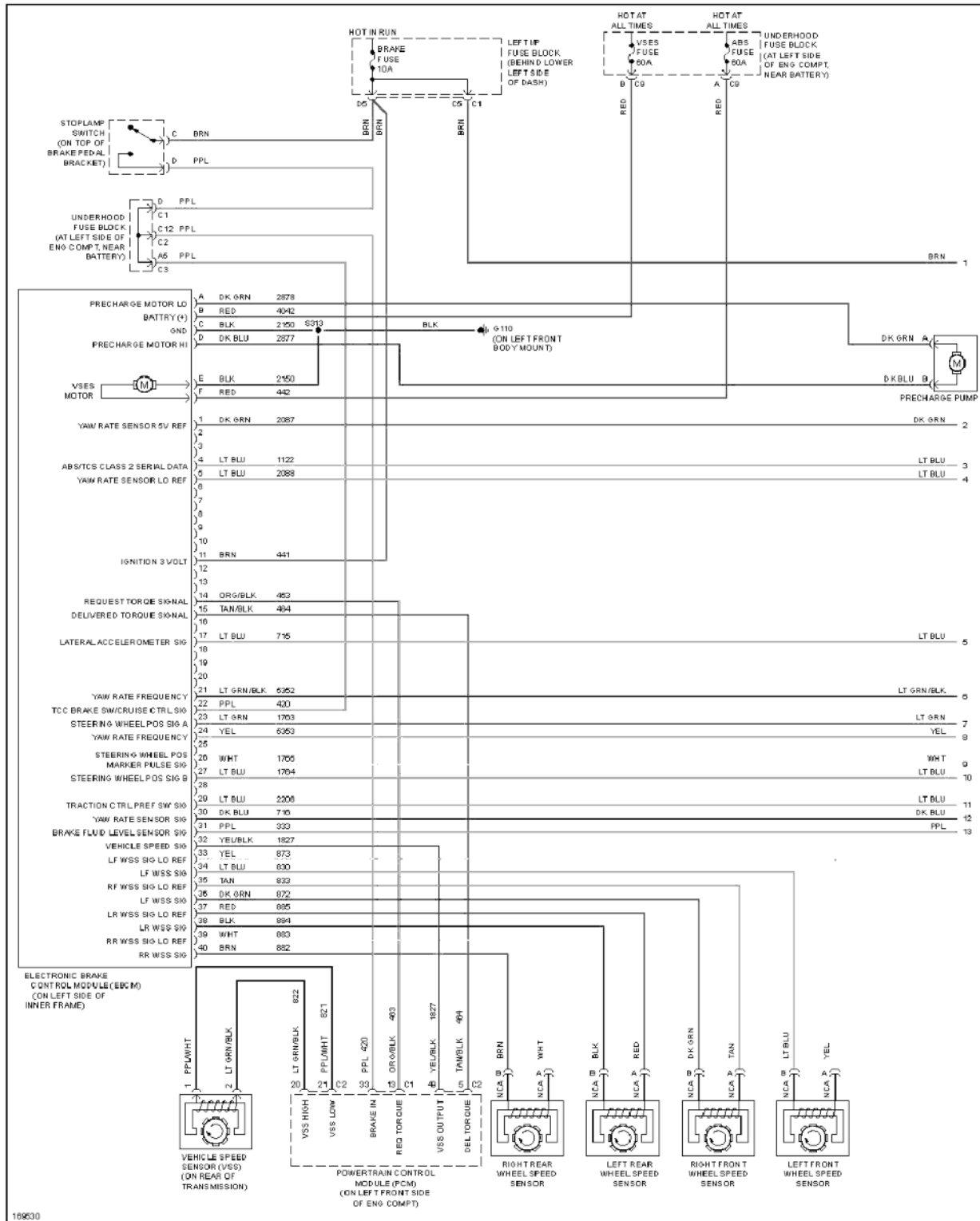
Fig. 9: Anti-lock Brakes Circuit, W/ Vehicle Speed Enhancement Stability (1 of 2)
