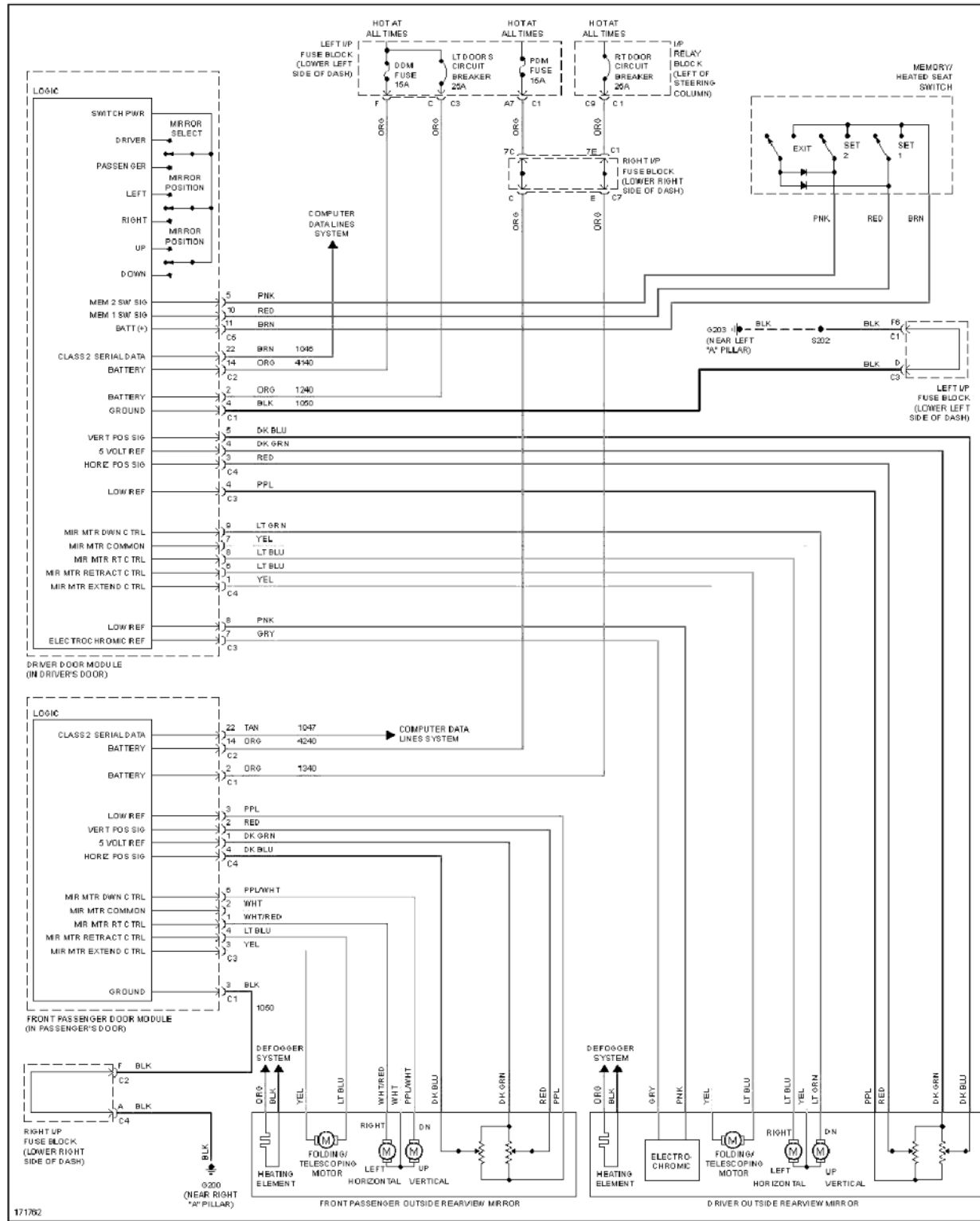
Fig. 63: Memory Mirrors Circuit
