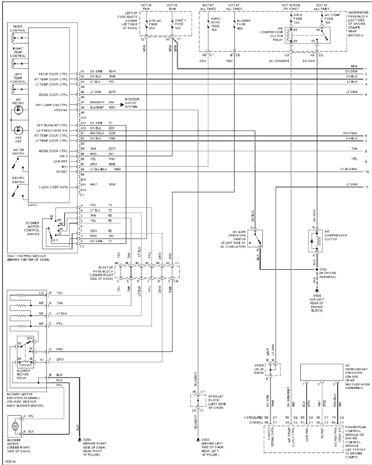
Fig. 5: Manual A/C Circuit (1 of 2)
