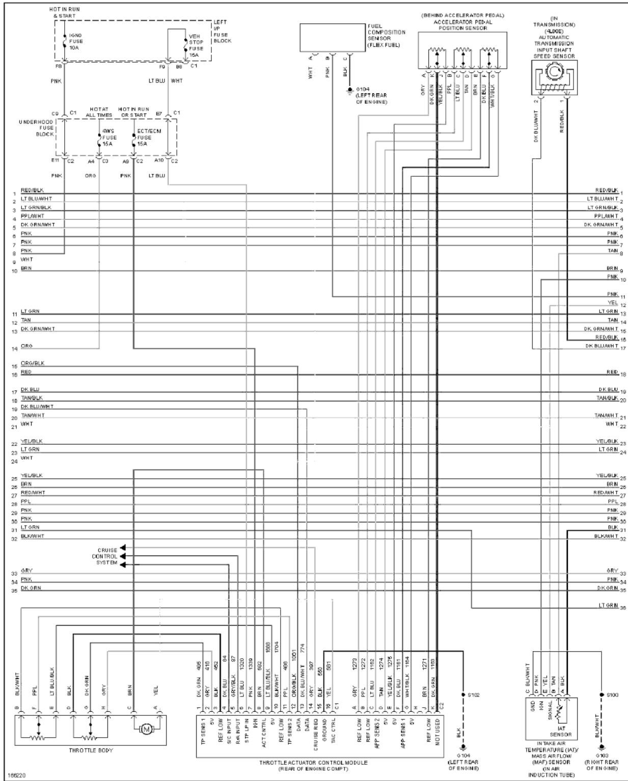
Fig. 36: 6.0L VIN U, Engine Performance Circuit (4 of 5)
