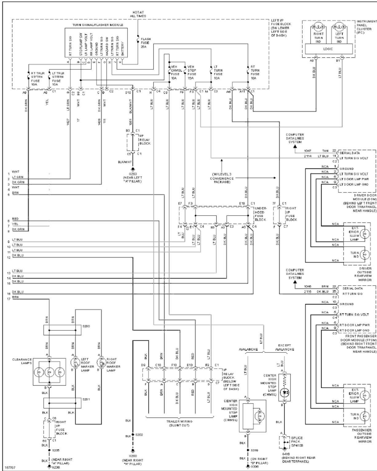
Fig. 46: Exterior Lamps Circuit (3 of 3)
