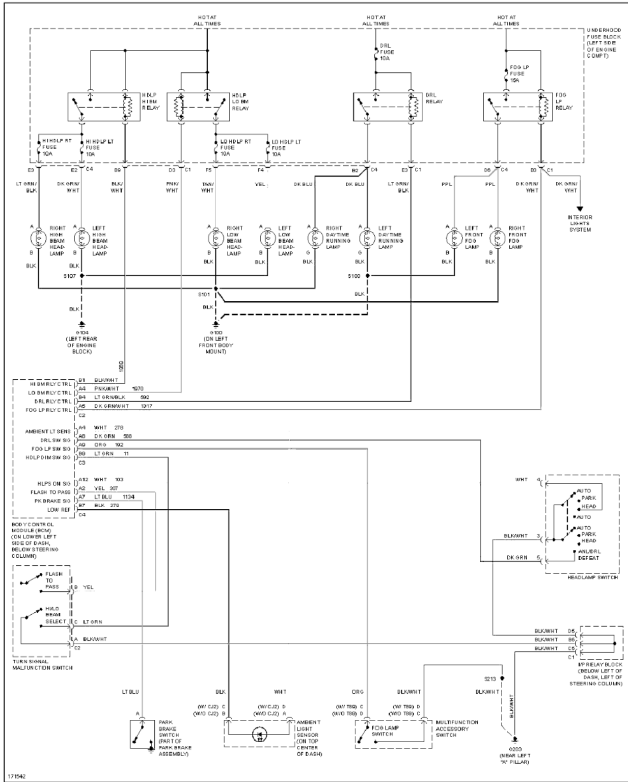
Fig. 52: Headlights Circuit
