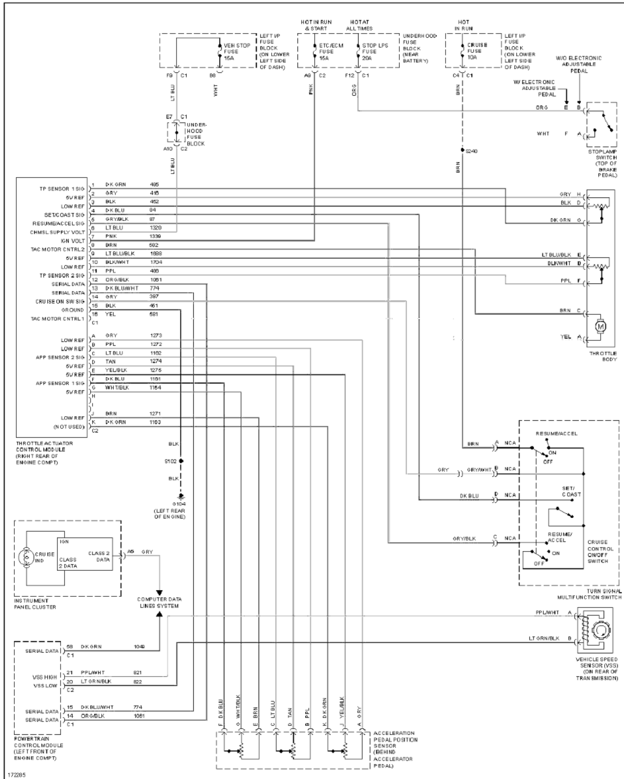
Fig. 18: Cruise Control Circuit
