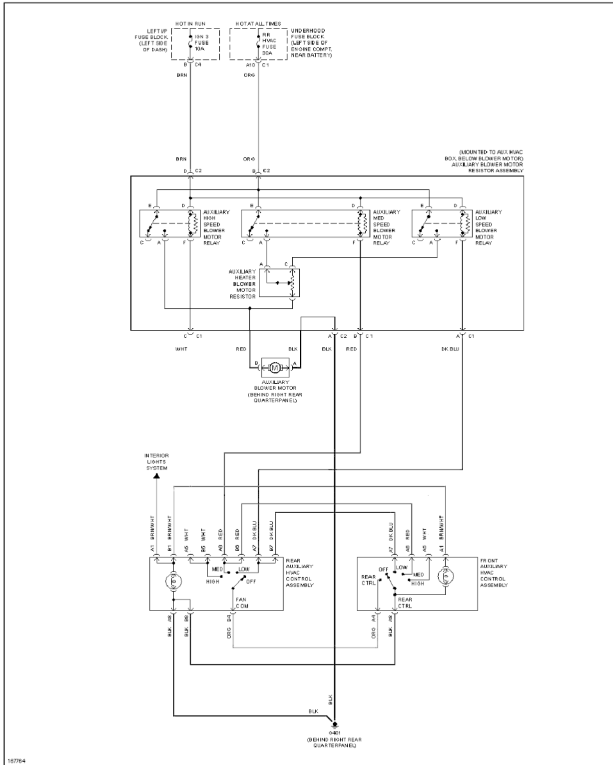
Fig. 7: Manual A/C Circuit, Rear W/ A/C only
