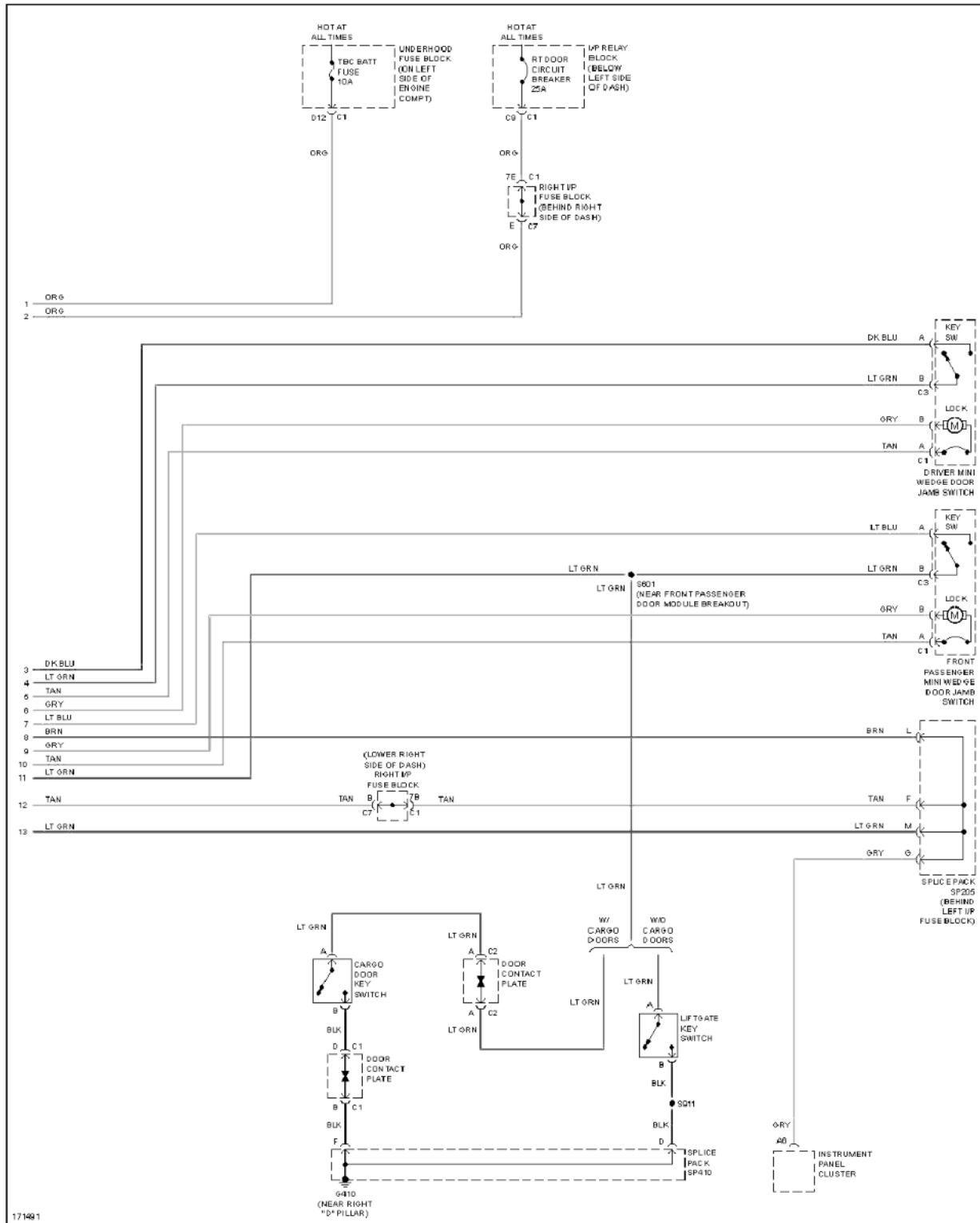
Fig. 73: Power Door Locks Circuit (2 of 2)
