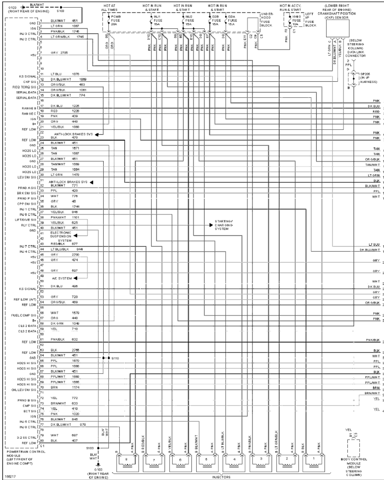
Fig. 23: 5.3L VIN T, Engine Performance Circuit (1 of 5)
