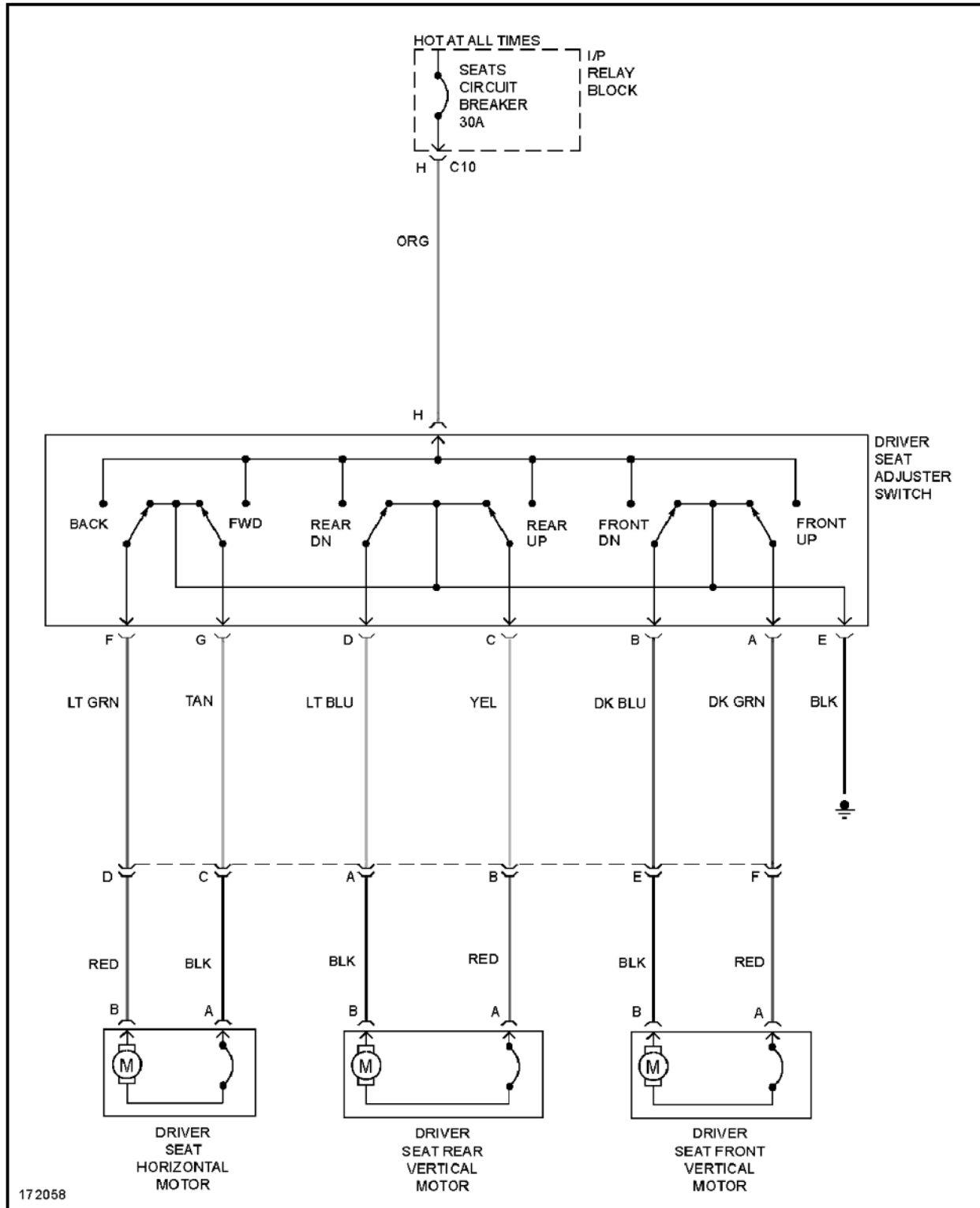
Fig. 76: Driver Seat Circuit
