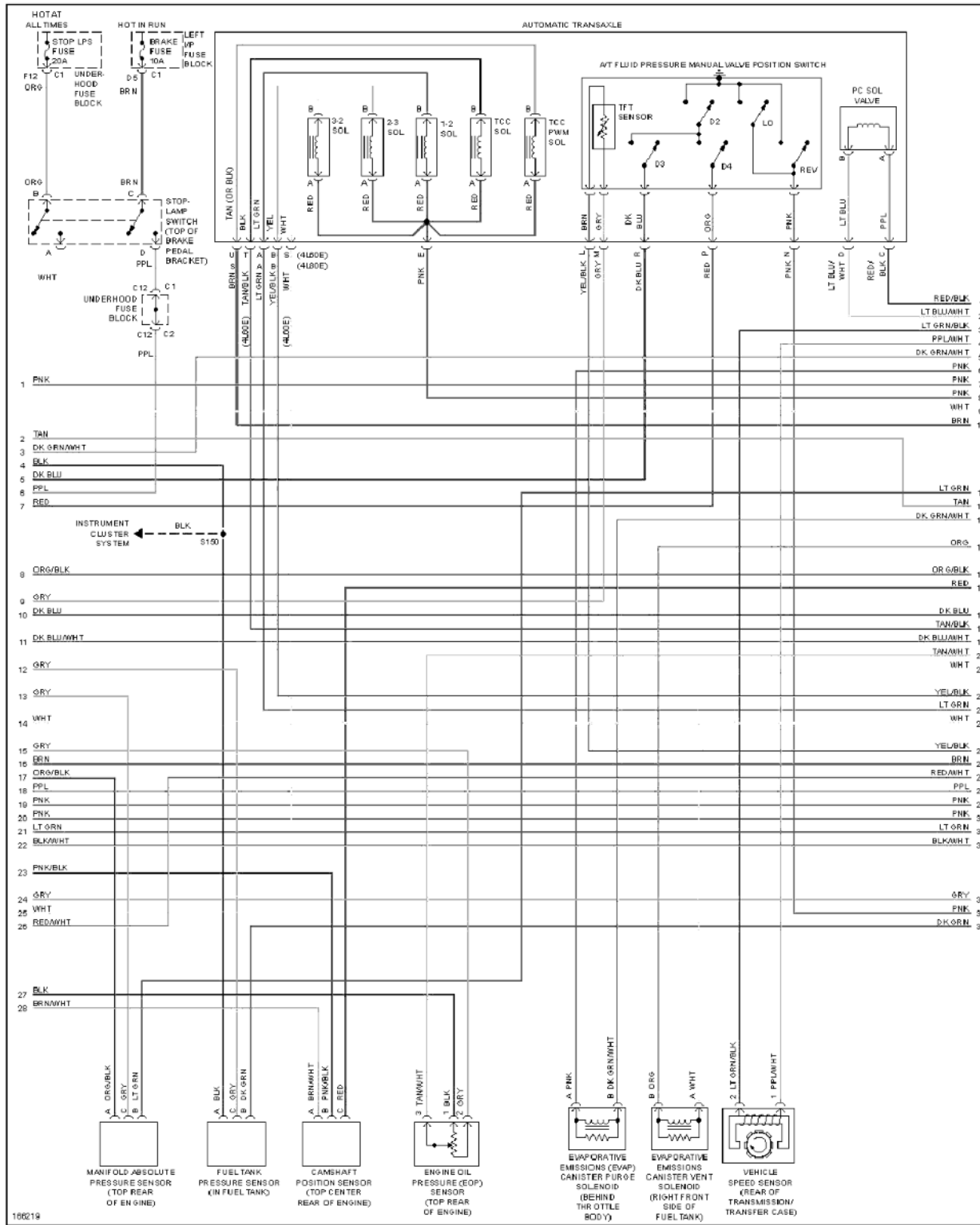
Fig. 25: 5.3L VIN T, Engine Performance Circuit (3 of 5)
