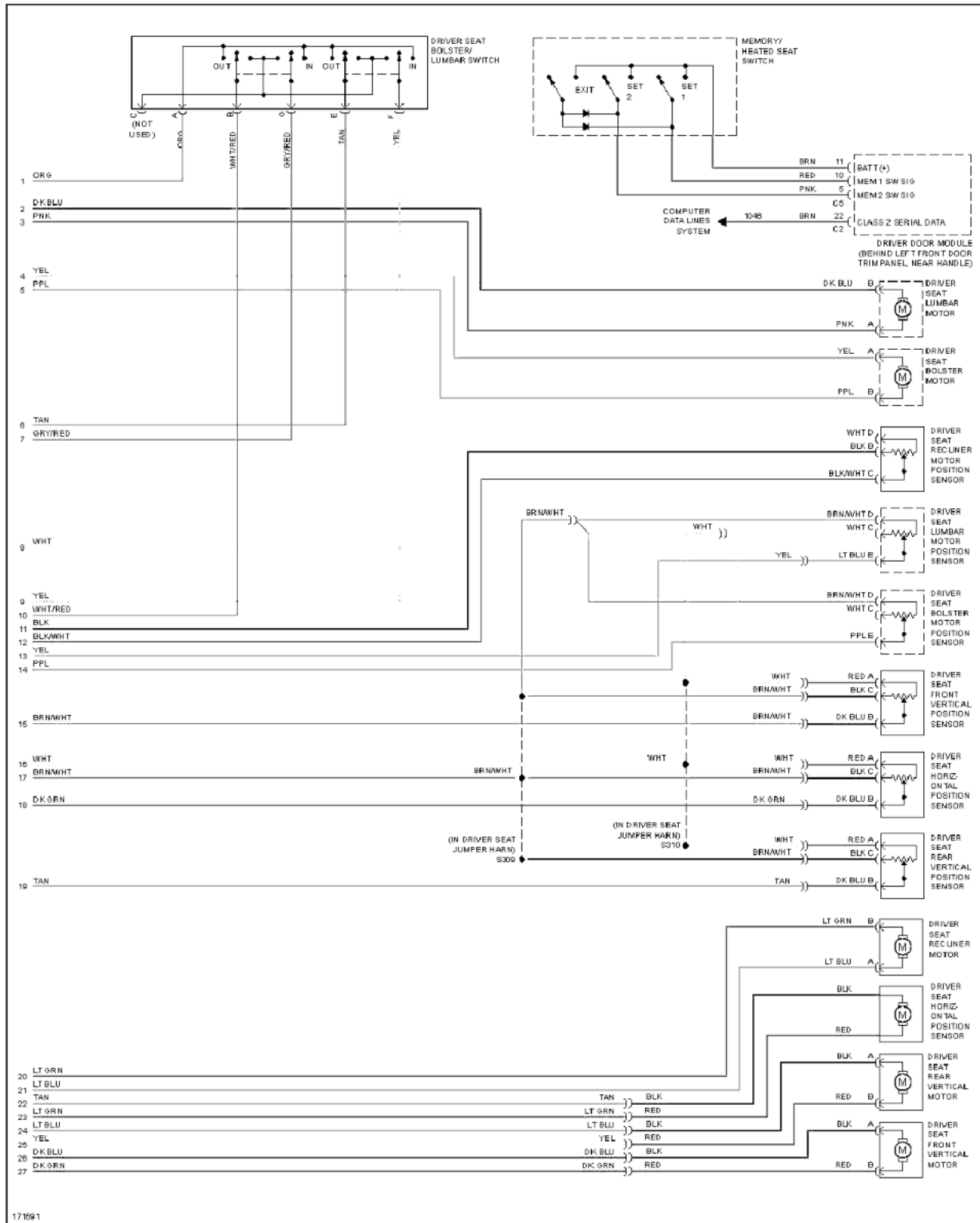
Fig. 65: Memory Seat Circuit (2 of 2)
