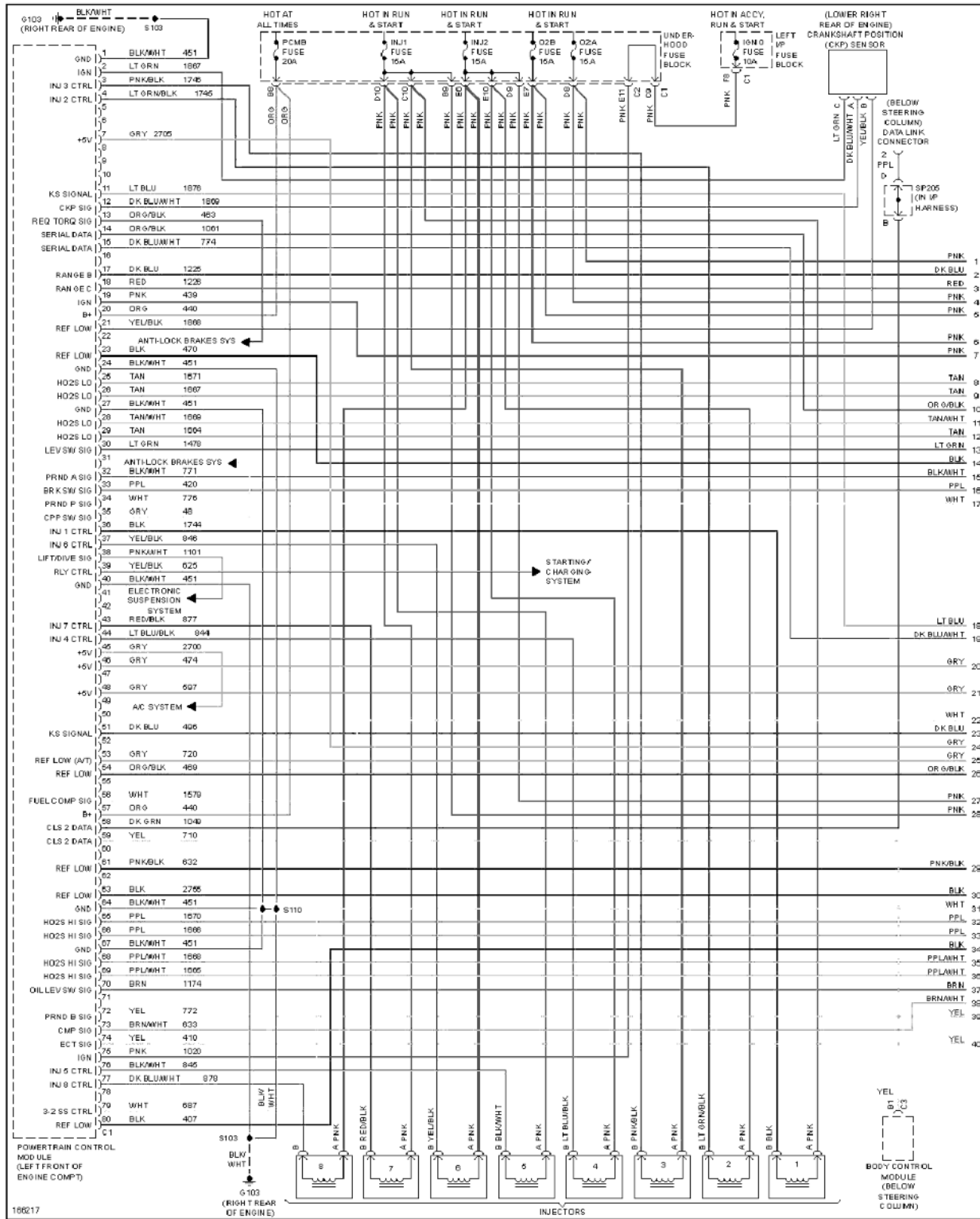
Fig. 28: 5.3L VIN Z, Engine Performance Circuit (1 of 5)
