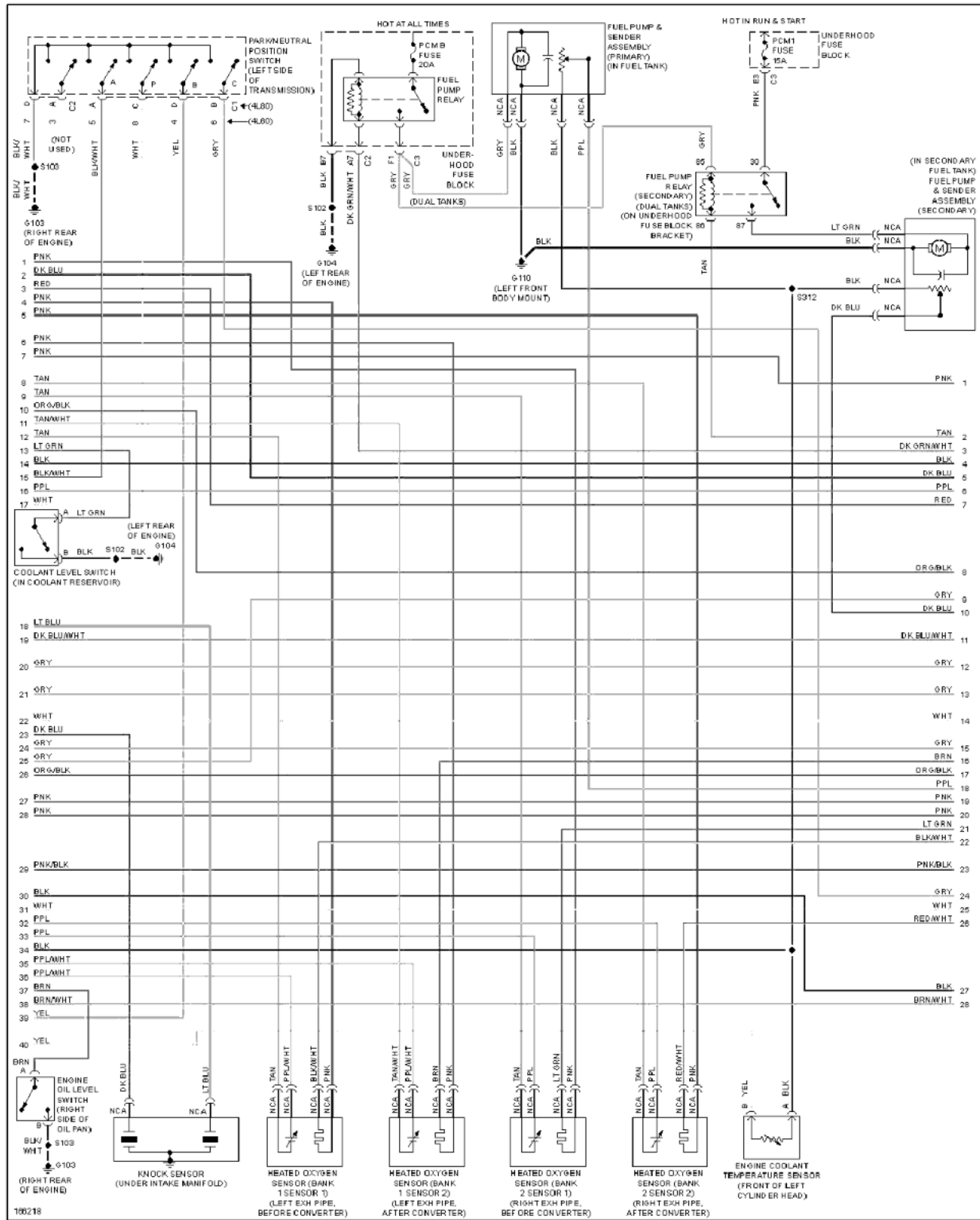
Fig. 24: 5.3L VIN T, Engine Performance Circuit (2 of 5)
