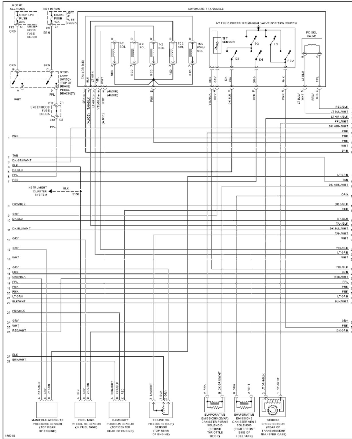
Fig. 30: 5.3L VIN Z, Engine Performance Circuit (3 of 5)
