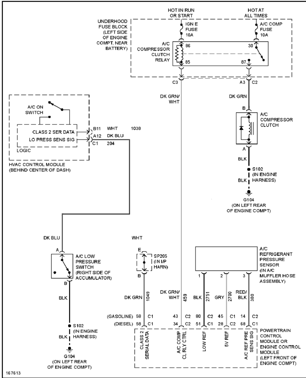
Fig. 4: Compressor Circuit
