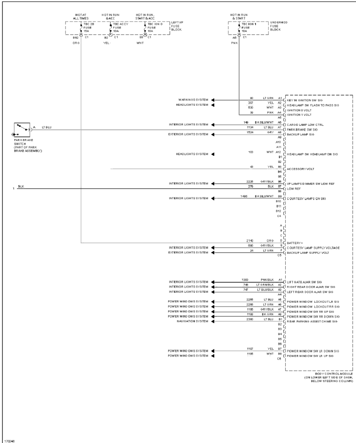
Fig. 15: Body Control Modules Circuit (2 of 2)
