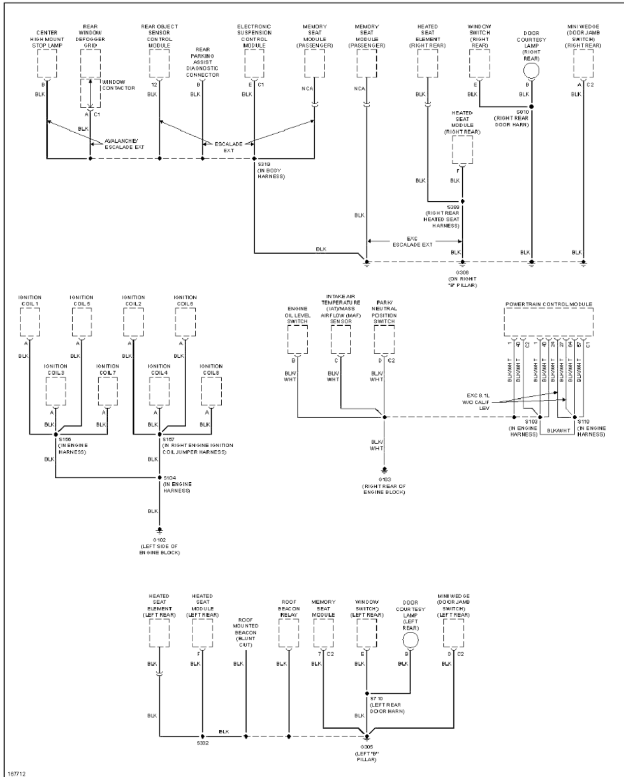
Fig. 48: Ground Distribution Circuit (2 of 5)
