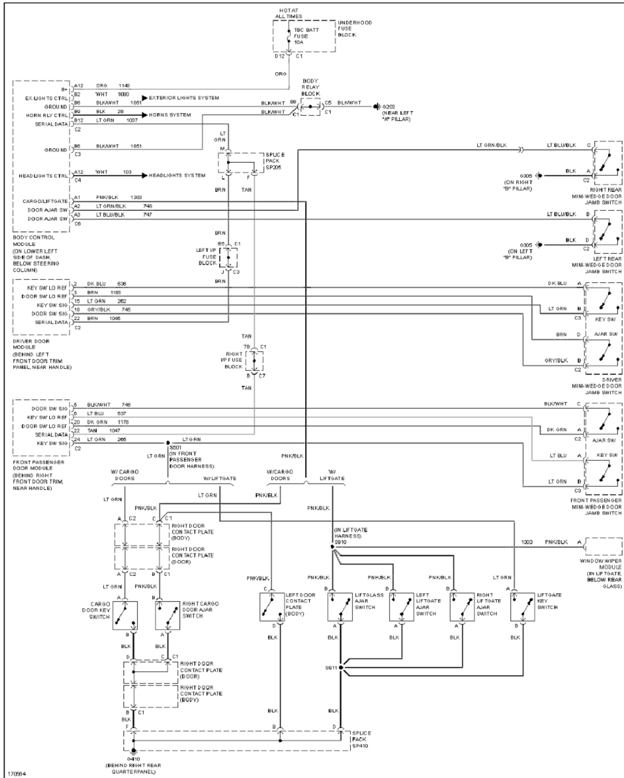
Fig. 12: Forced Entry Circuit
