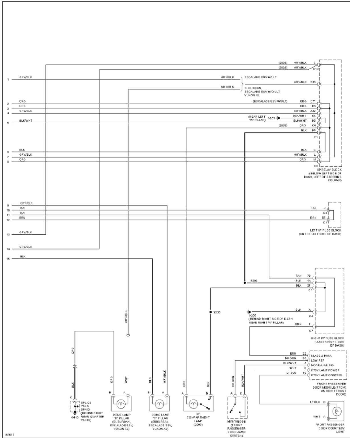
Fig. 58: Courtesy Lamps Circuit (3 of 3)
