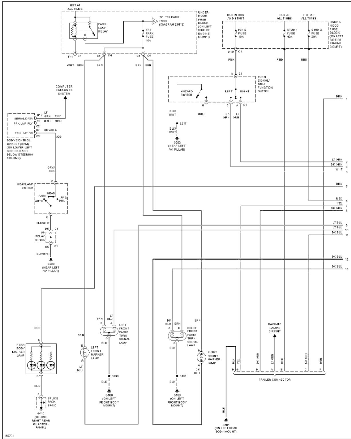
Fig. 44: Exterior Lamps Circuit (1 of 3)
