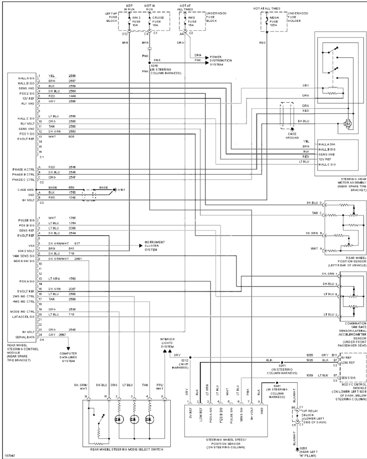
Fig. 21: Rear Wheel Steering Circuit ELECTRONIC SUSPENSION
