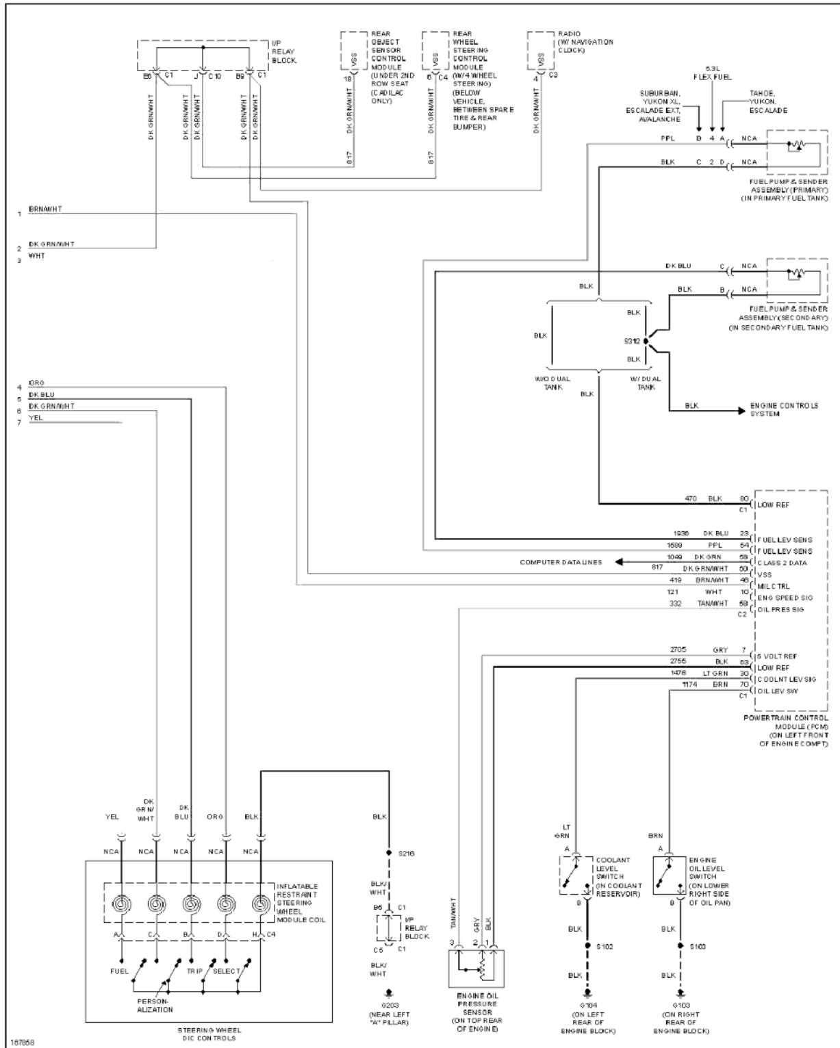
Fig. 55: Instrument Cluster Circuit (2 of 2)
