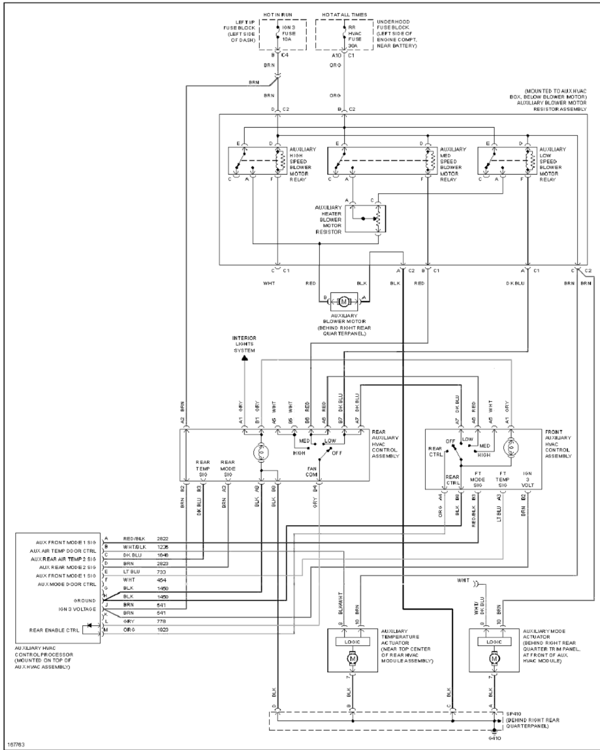
Fig. 8: Manual A/C Circuit, Rear W/ Heat & A/C
