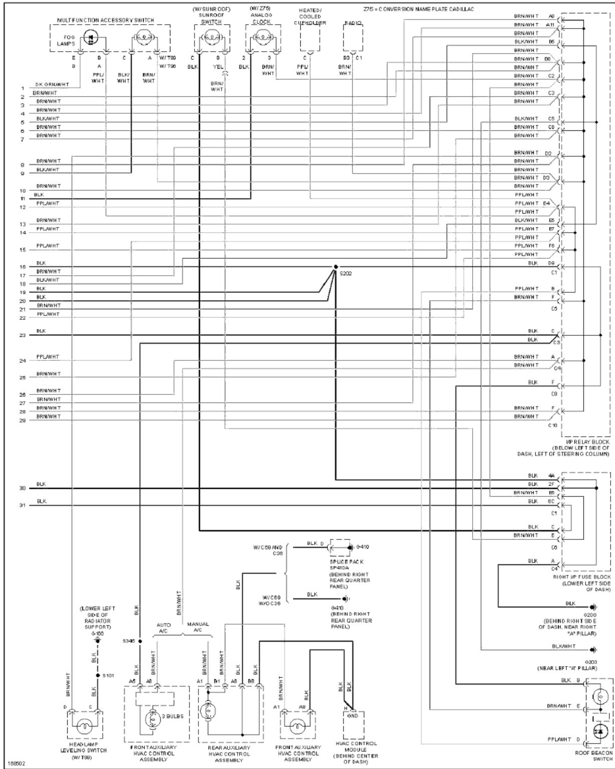
Fig. 61: Instrument Illumination Circuit (3 of 3)
