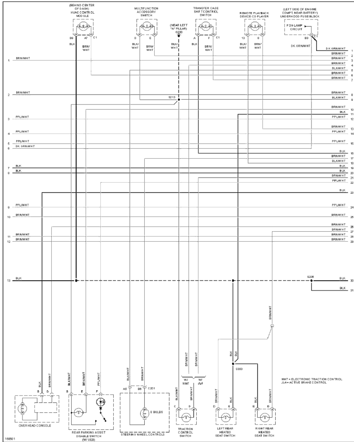
Fig. 60: Instrument Illumination Circuit (2 of 3)
