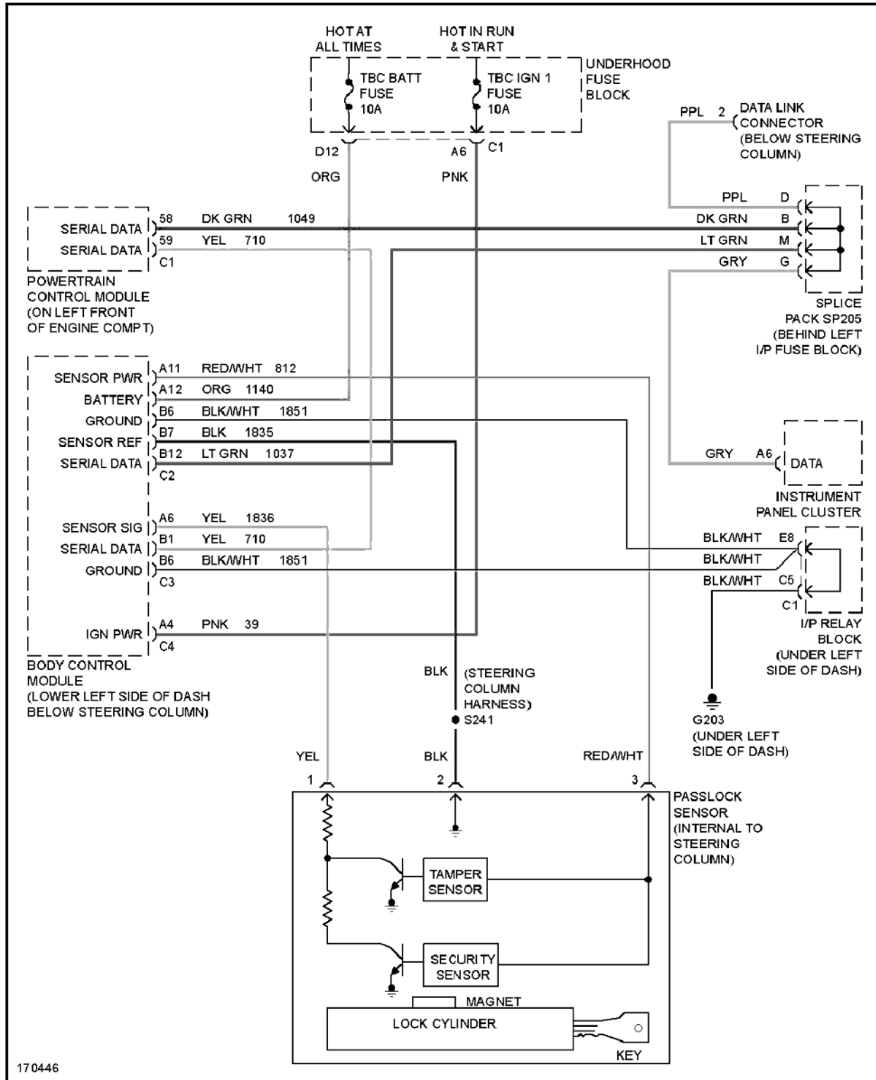
Fig. 13: Passlock Circuit
