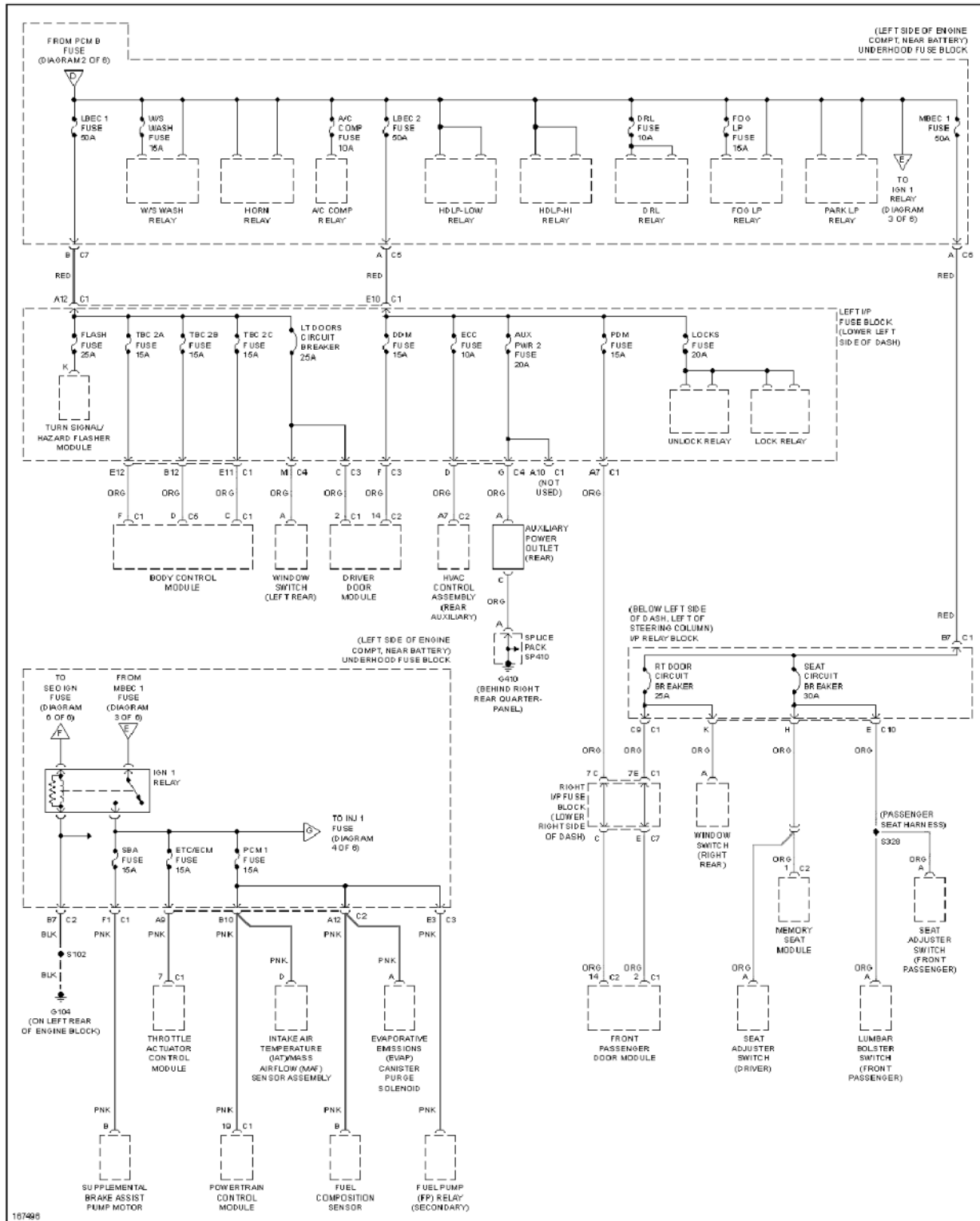
Fig. 68: Power Distribution Circuit (3 of 6)
