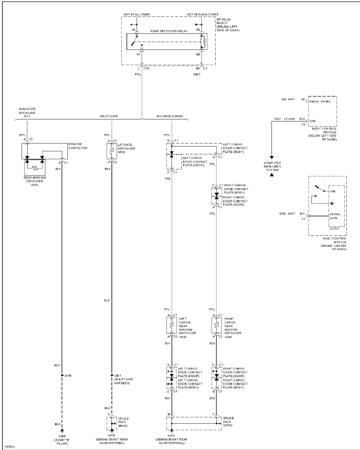
Fig. 20: Rear Defogger Circuit
