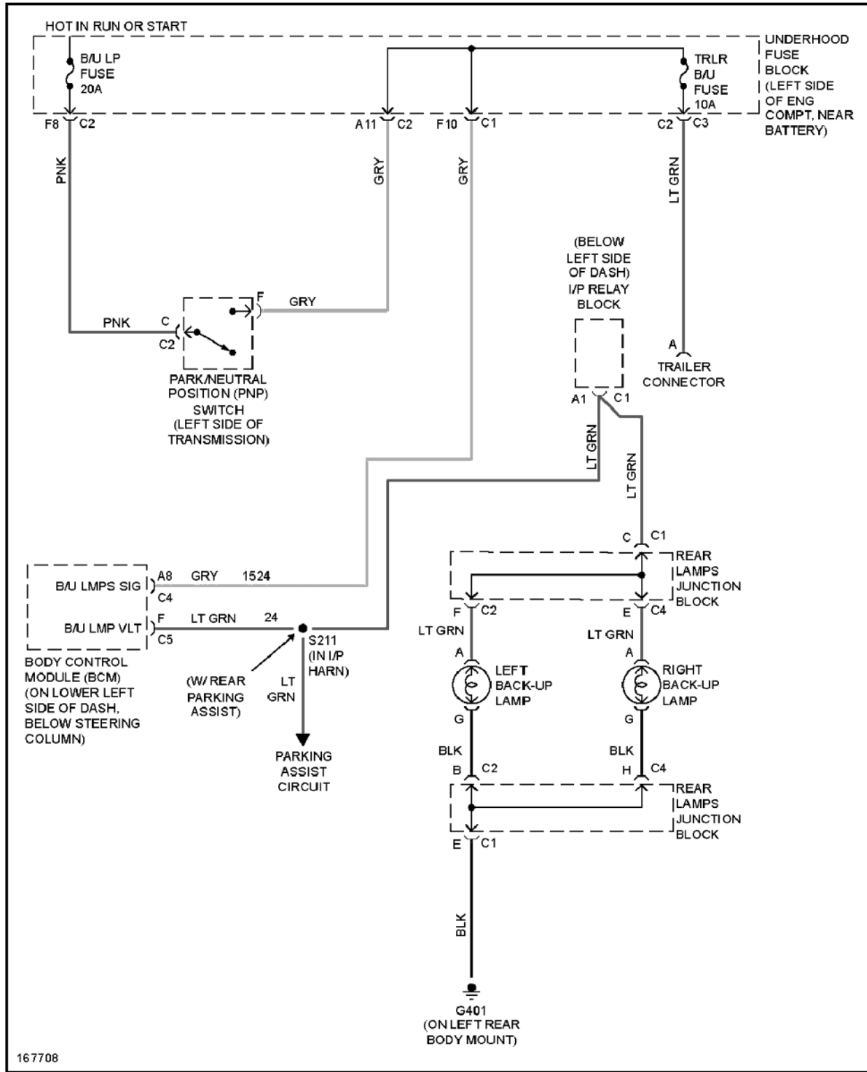
Fig. 43: Back-up Lamps Circuit
