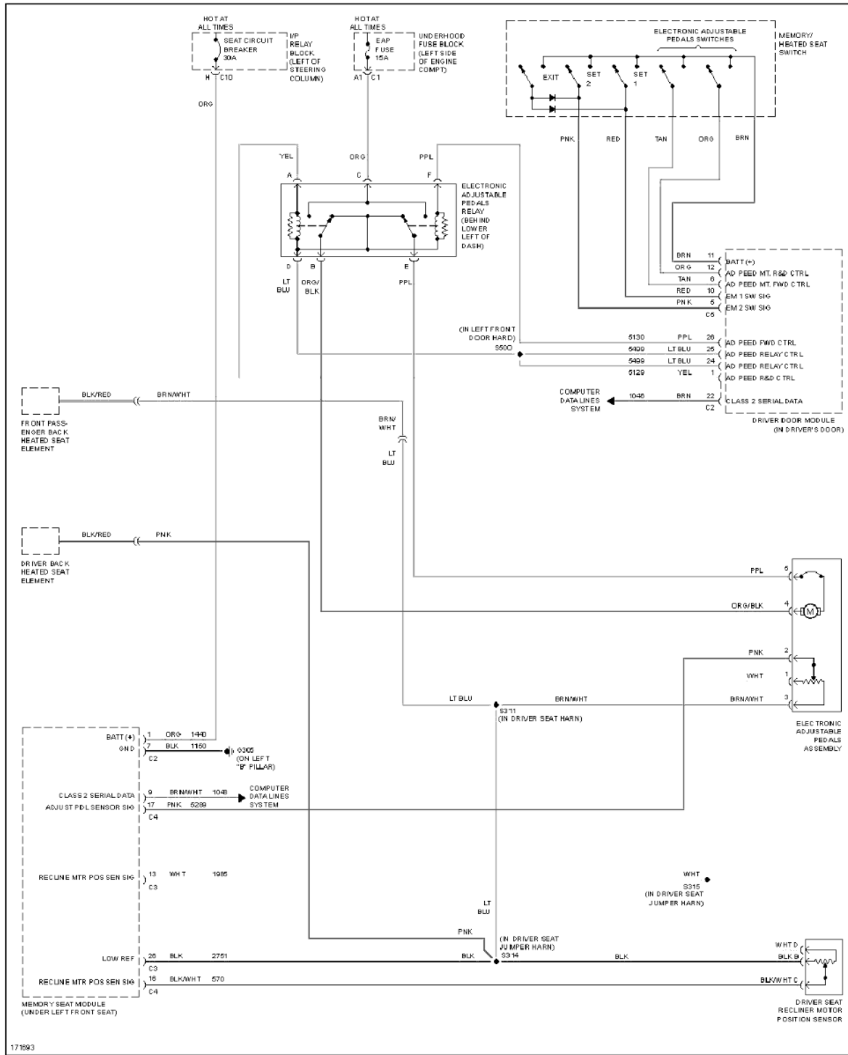
Fig. 62: Adjustable Pedal Circuit
