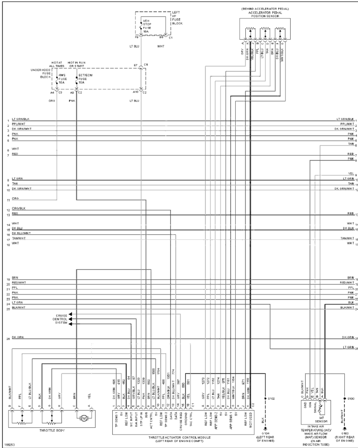
Fig. 41: 8.1L VIN G, Engine Performance Circuit (4 of 5)
