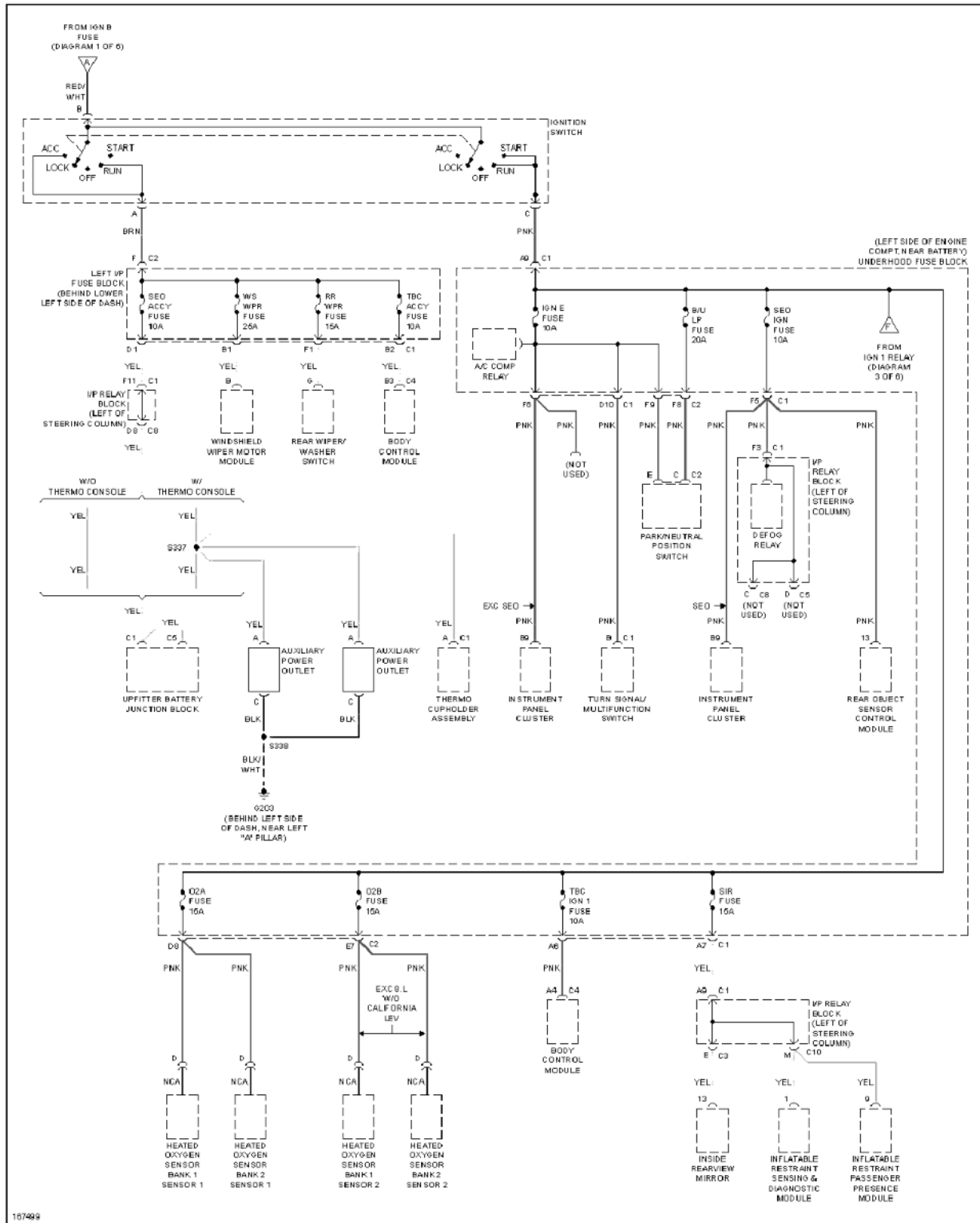
Fig. 71: Power Distribution Circuit (6 of 6)
