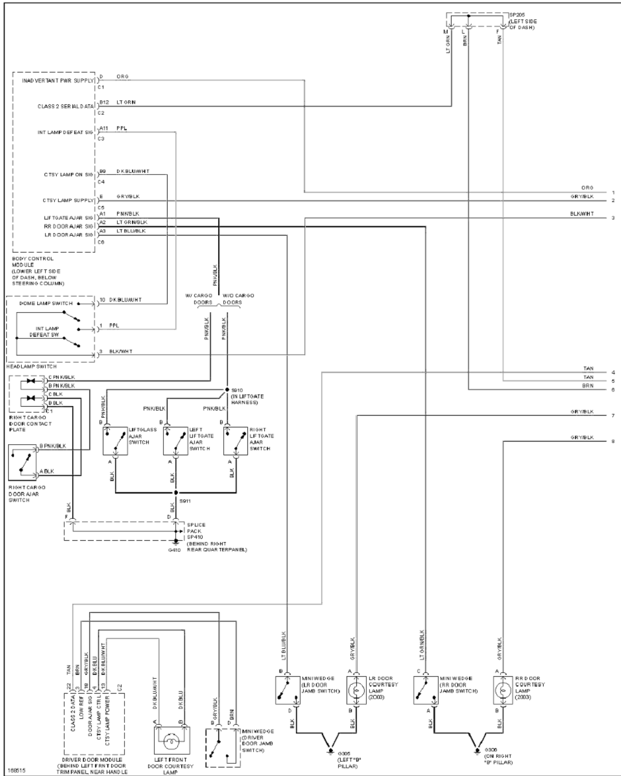
Fig. 56: Courtesy Lamps Circuit (1 of 3)
