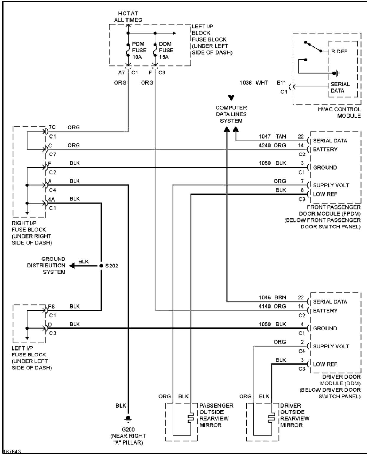
Fig. 19: Heated Mirrors Circuit
