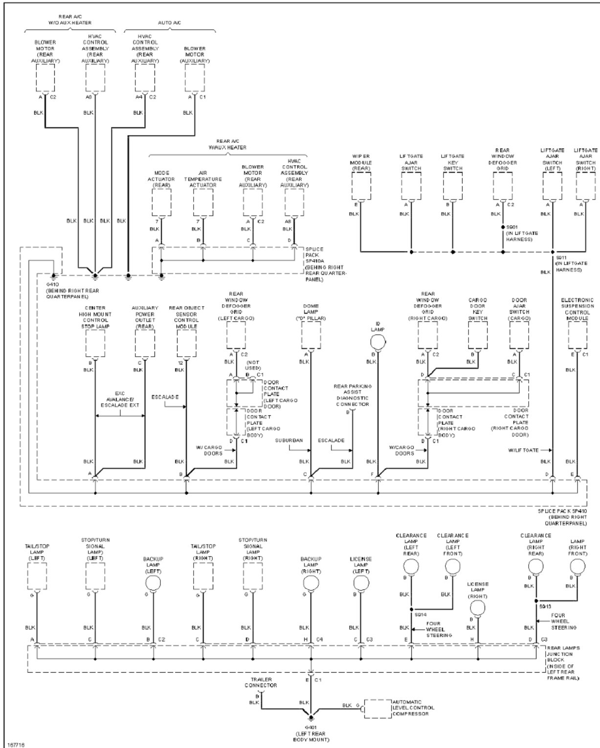
Fig. 51: Ground Distribution Circuit (5 of 5)
