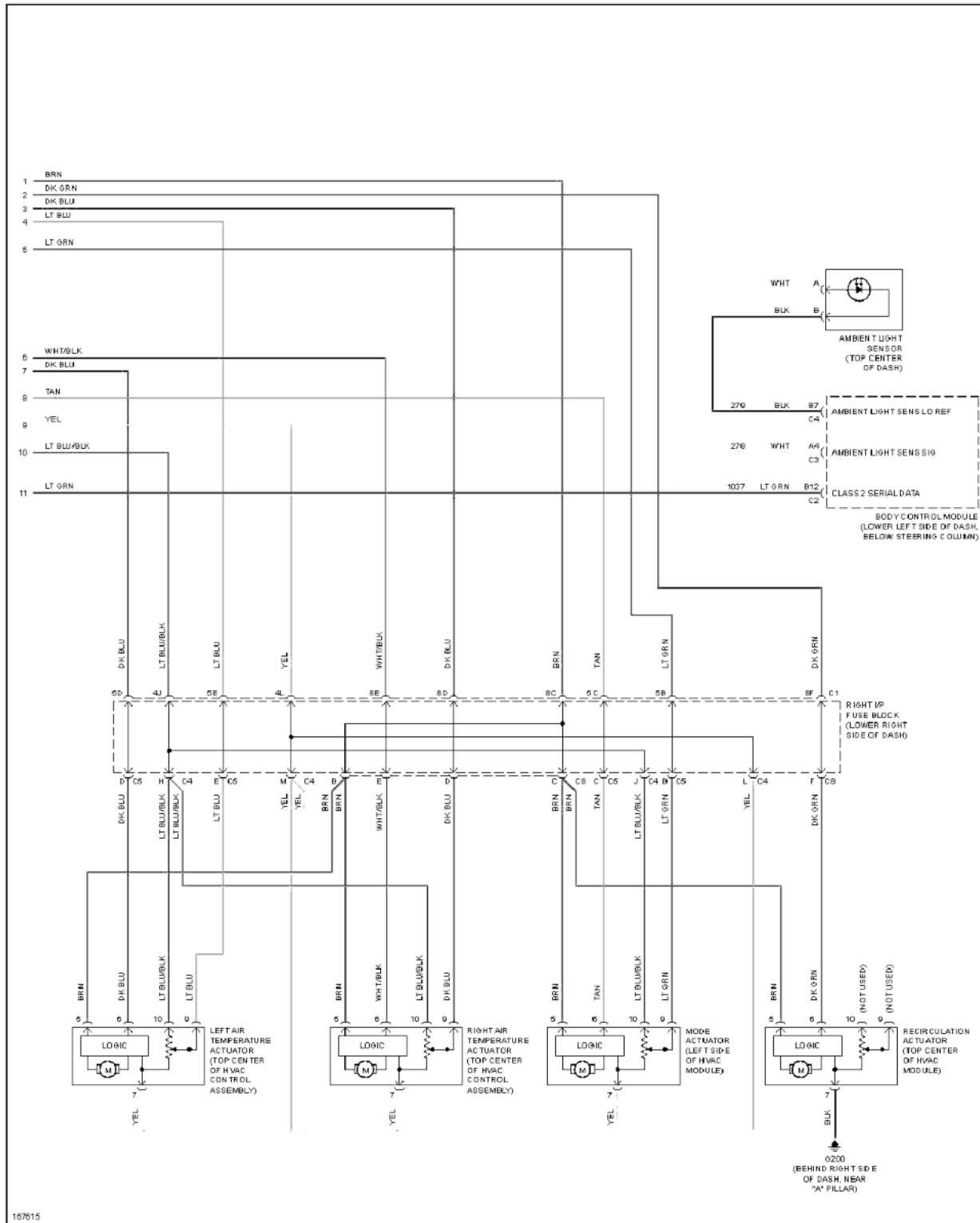
Fig. 6: Manual A/C Circuit (2 of 2)
