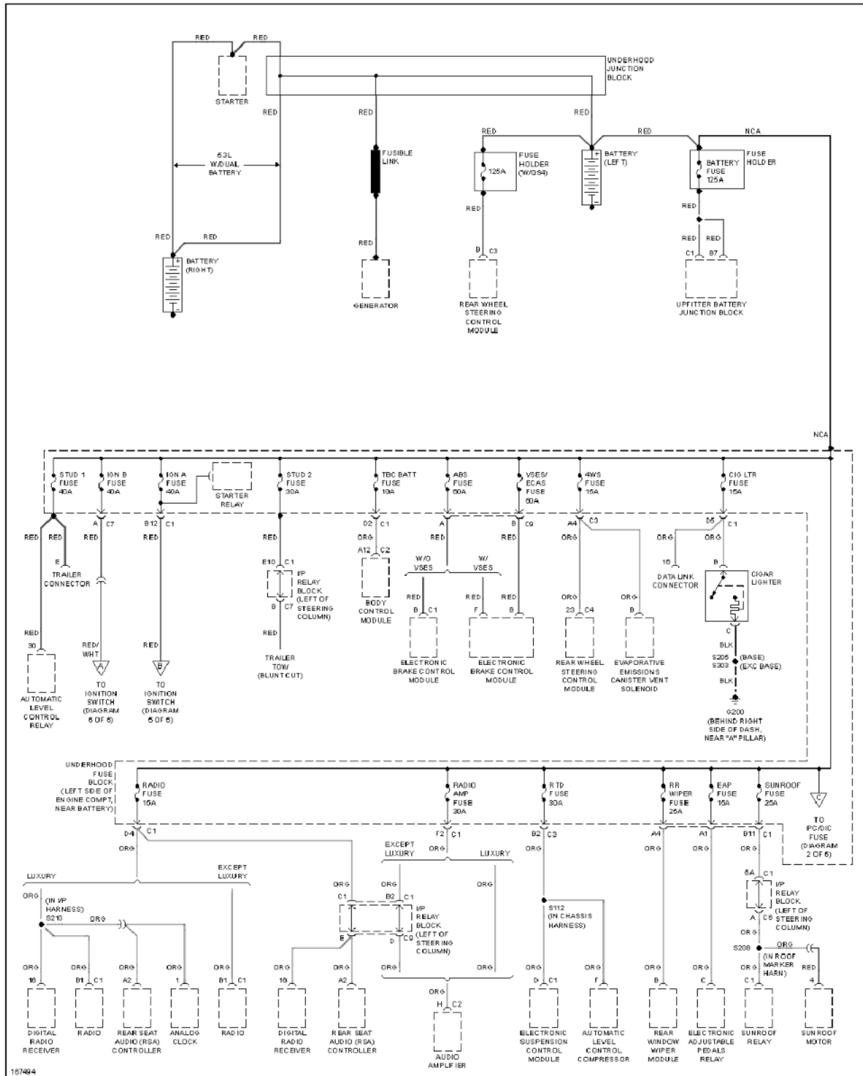
Fig. 66: Power Distribution Circuit (1 of 6)
