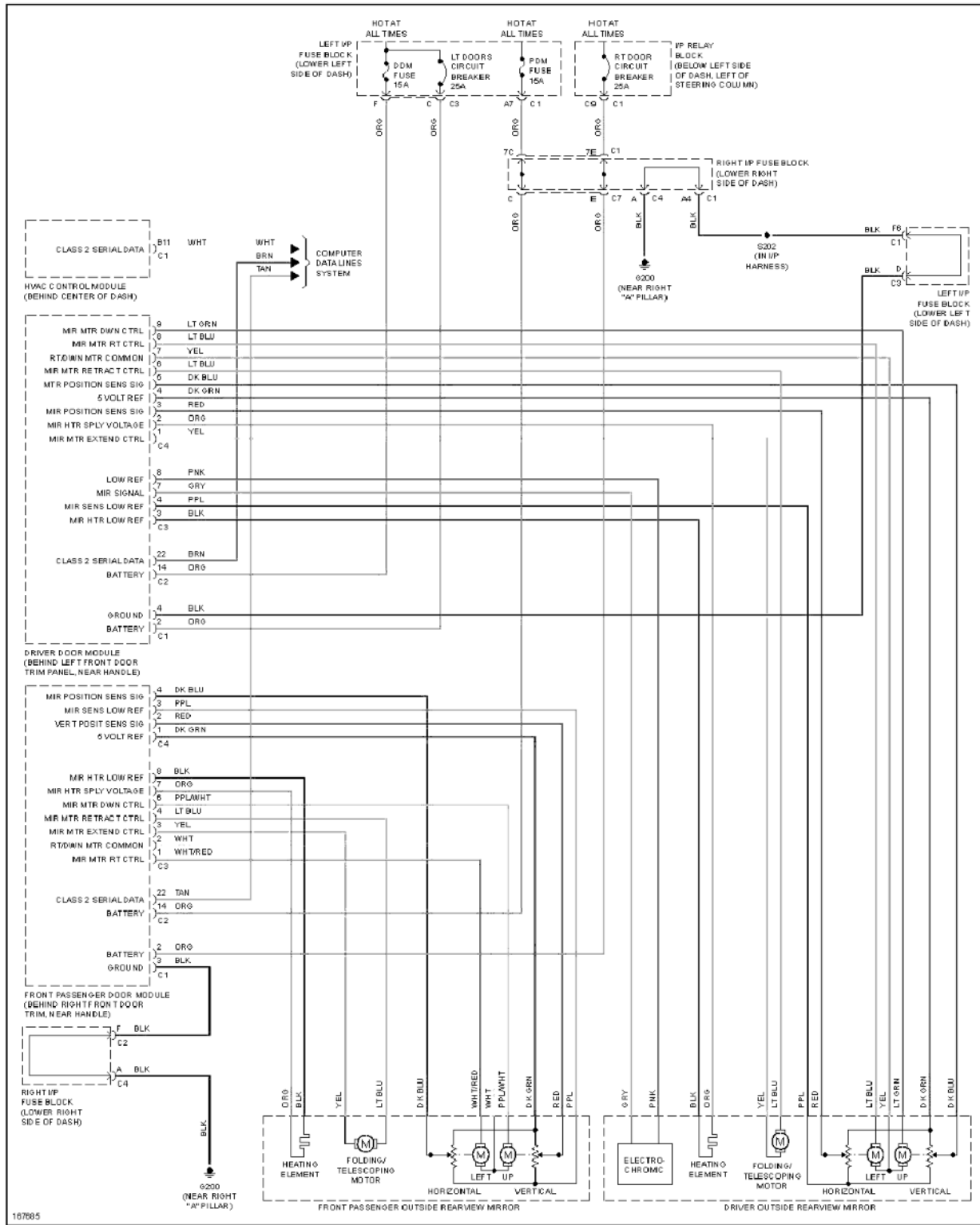
Fig. 75: Power Mirrors Circuit
