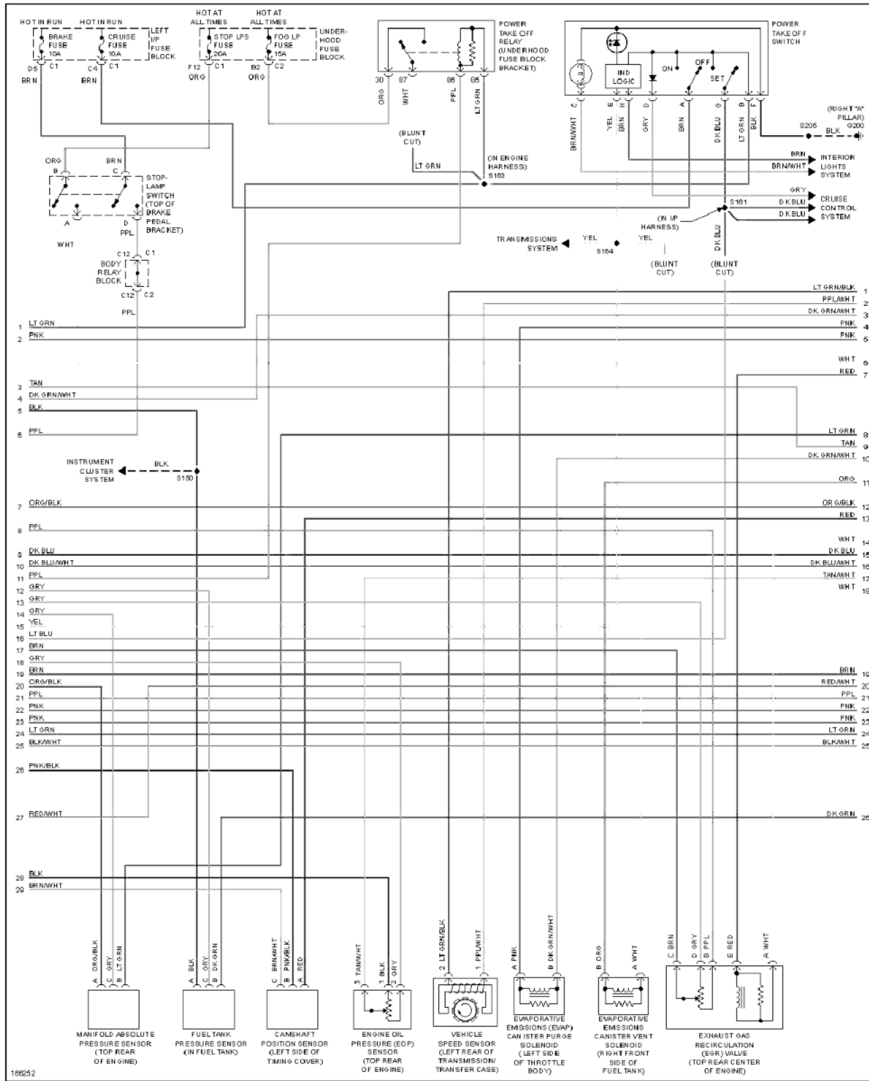
Fig. 40: 8.1L VIN G, Engine Performance Circuit (3 of 5)
