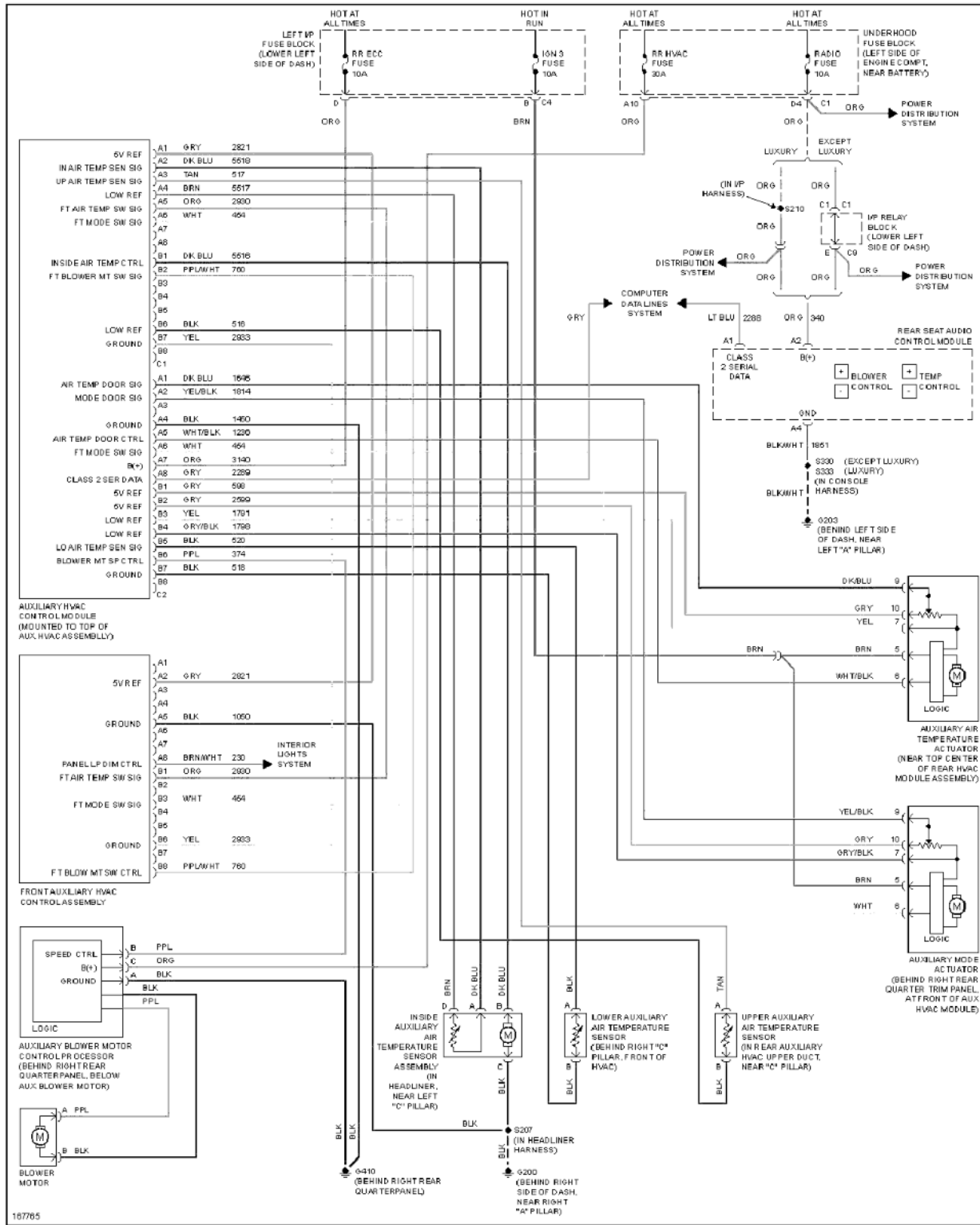
Fig. 3: Automatic A/C Circuit, Rear A/C
