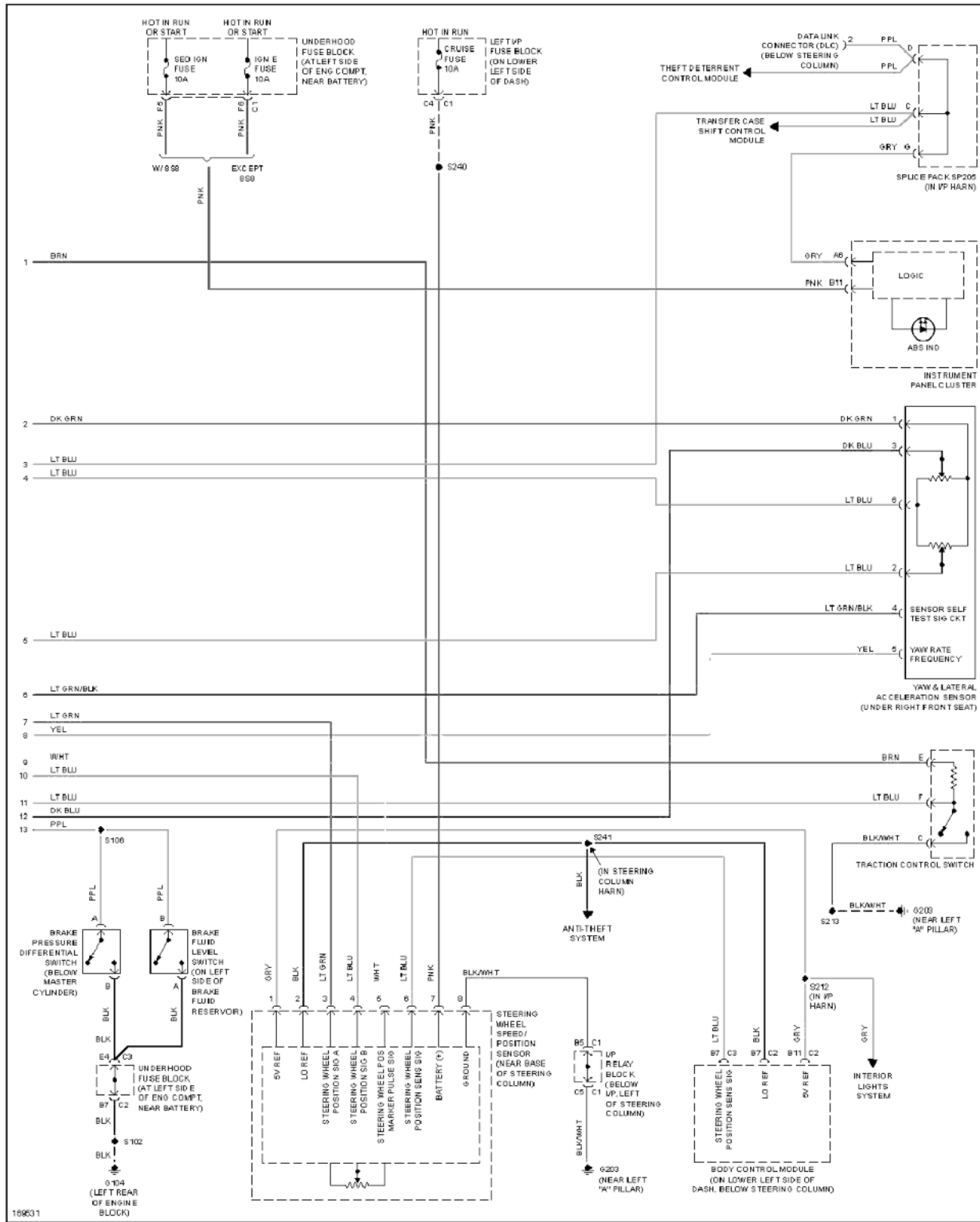
Fig. 10: Anti-lock Brakes Circuit, W/ Vehicle Speed Enhancement Stability (2 of 2)
