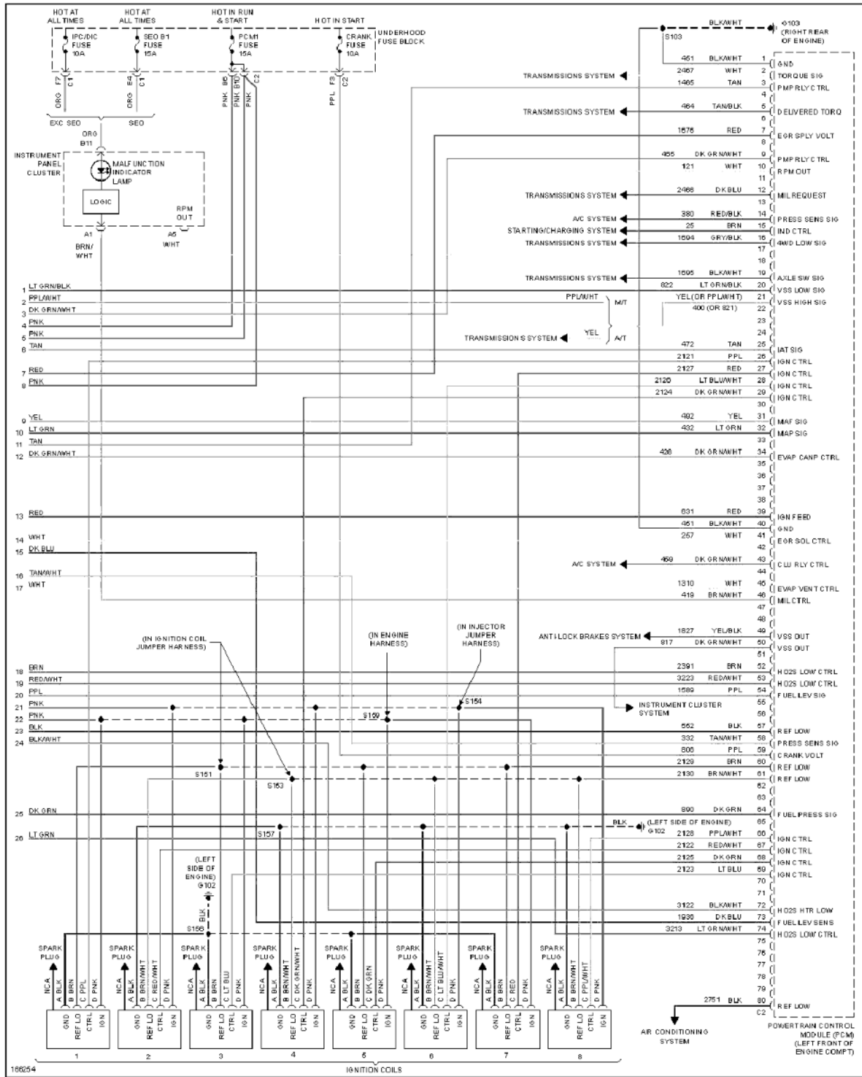
Fig. 42: 8.1L VIN G, Engine Performance Circuit (5 of 5)
