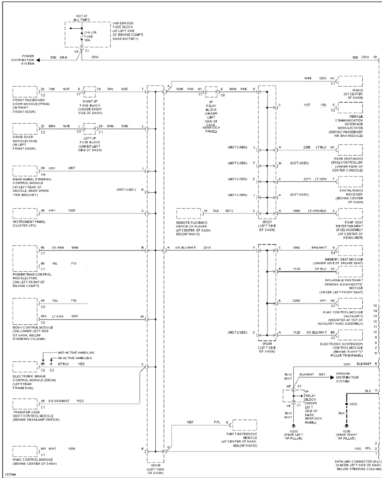
Fig. 16: Computer Data Lines Circuit, Base & Up-Level
