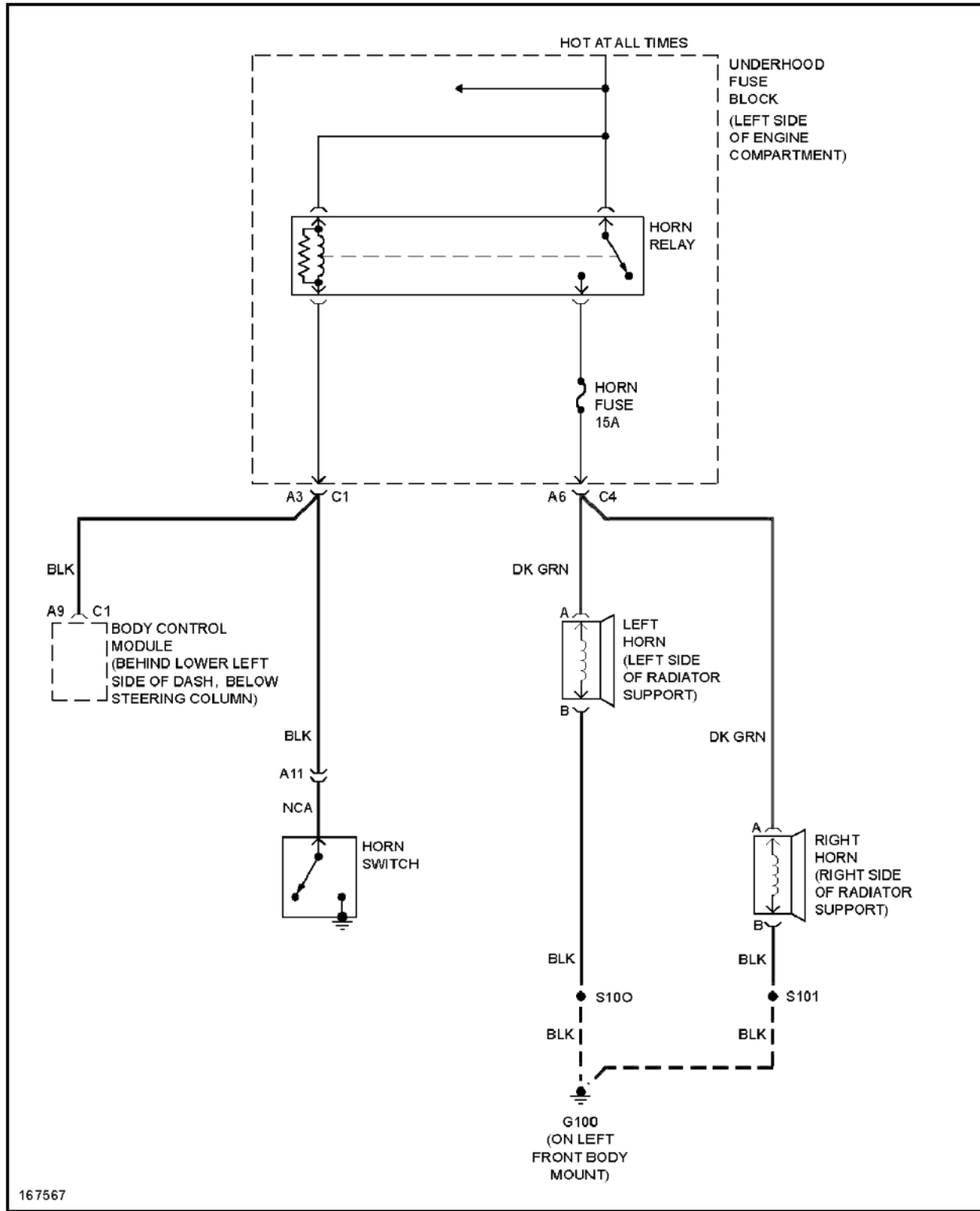
Fig. 53: Horn Circuit
