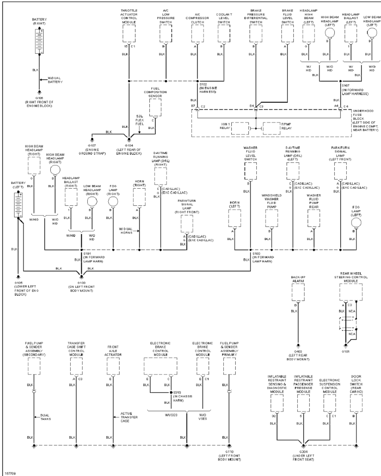
Fig. 47: Ground Distribution Circuit (1 of 5)
