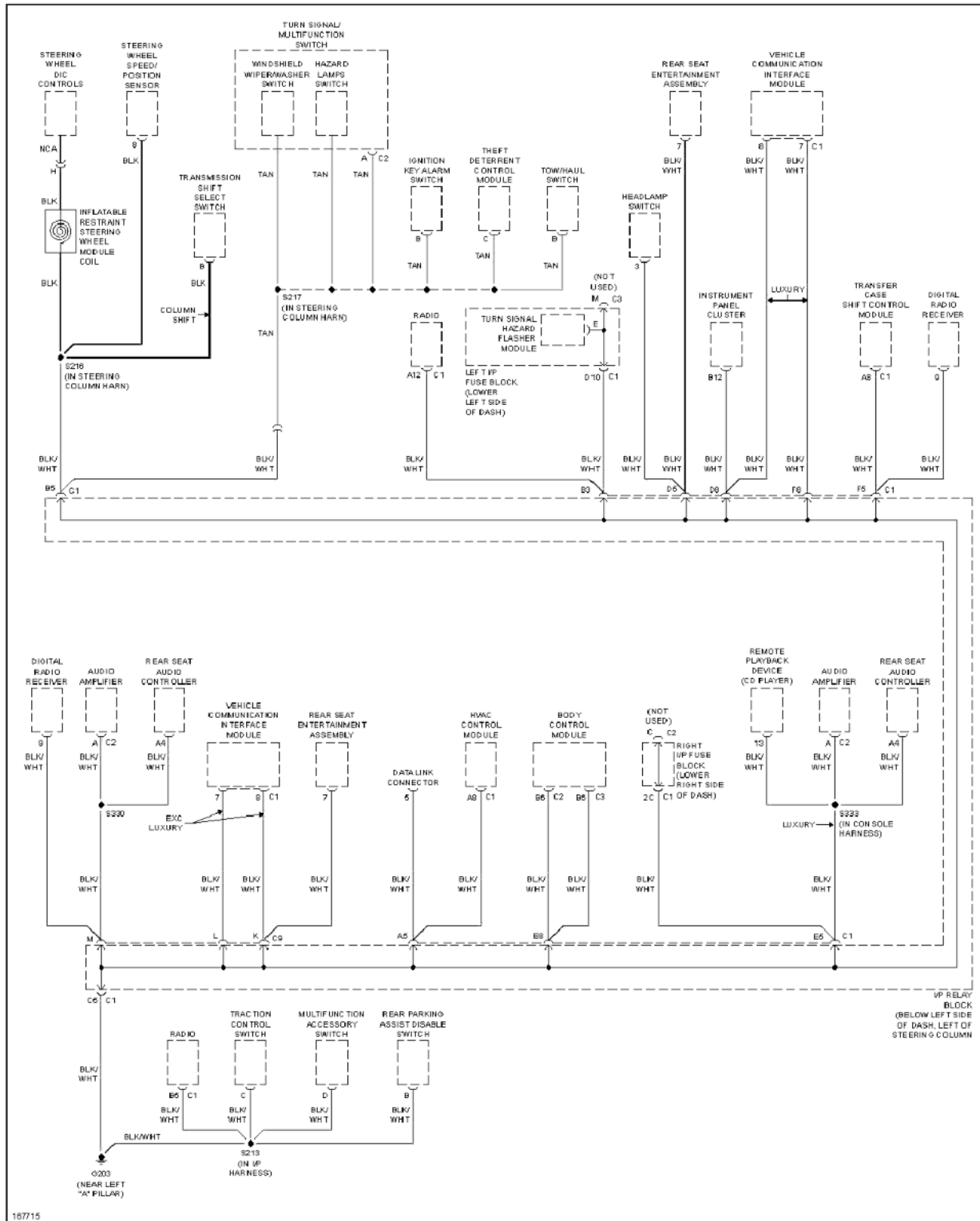
Fig. 50: Ground Distribution Circuit (4 of 5)
