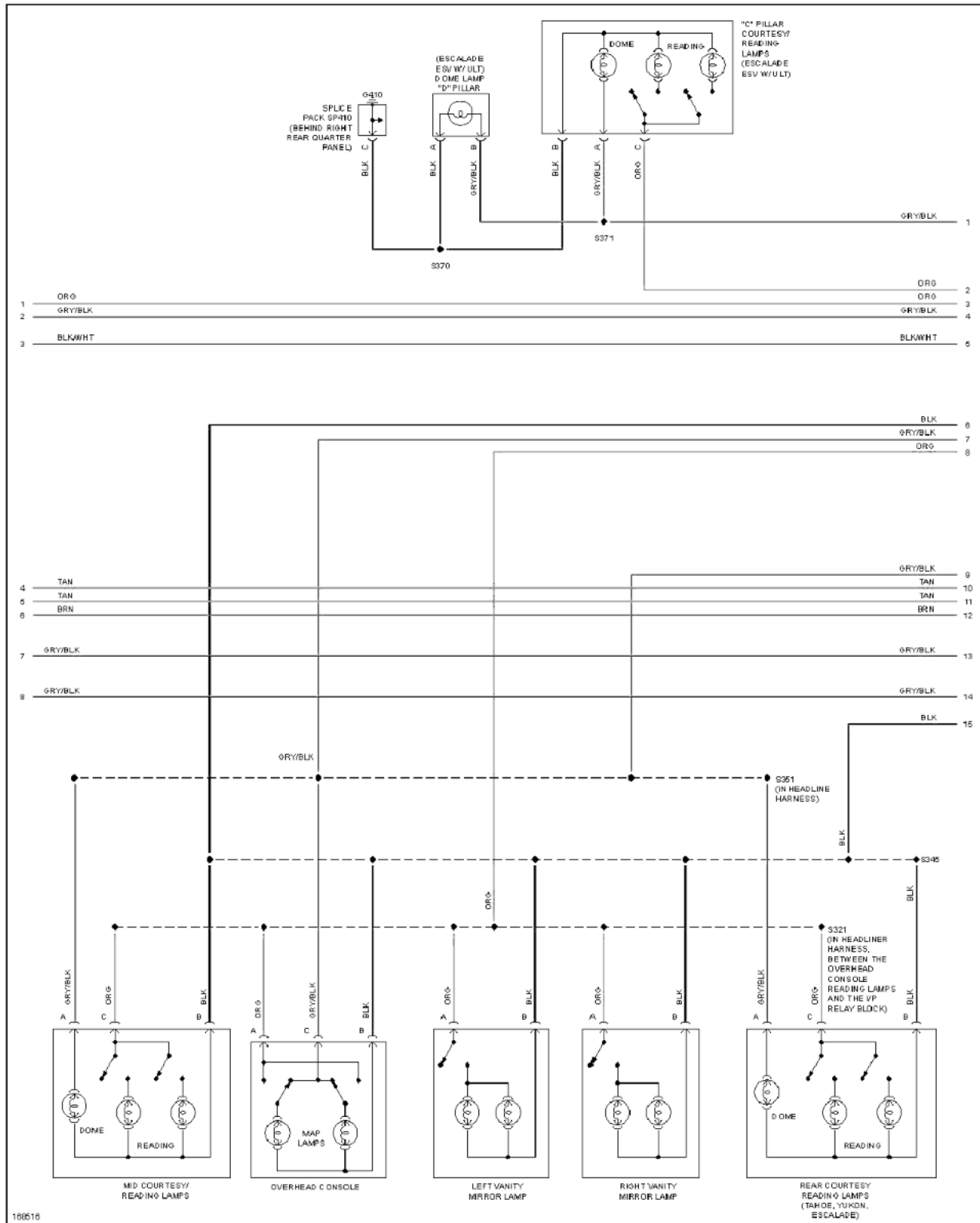
Fig. 57: Courtesy Lamps Circuit (2 of 3)
