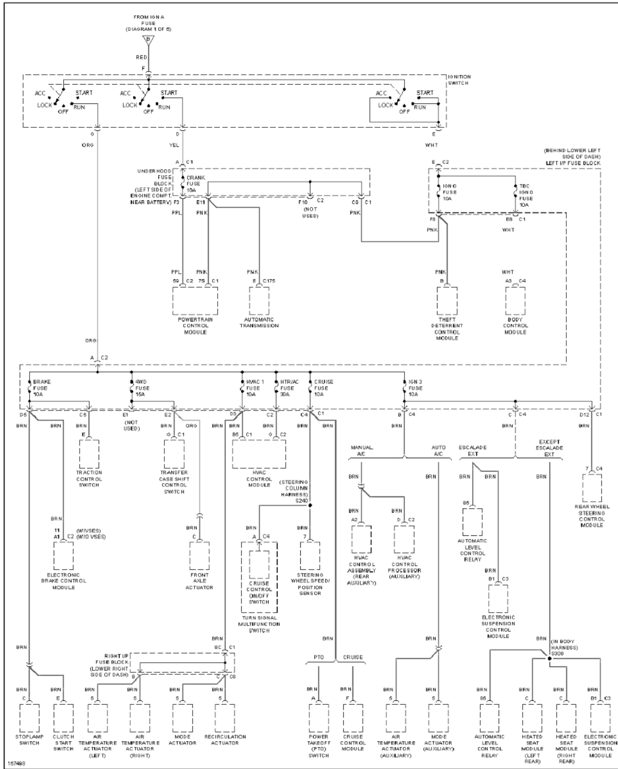
Fig. 70: Power Distribution Circuit (5 of 6)
