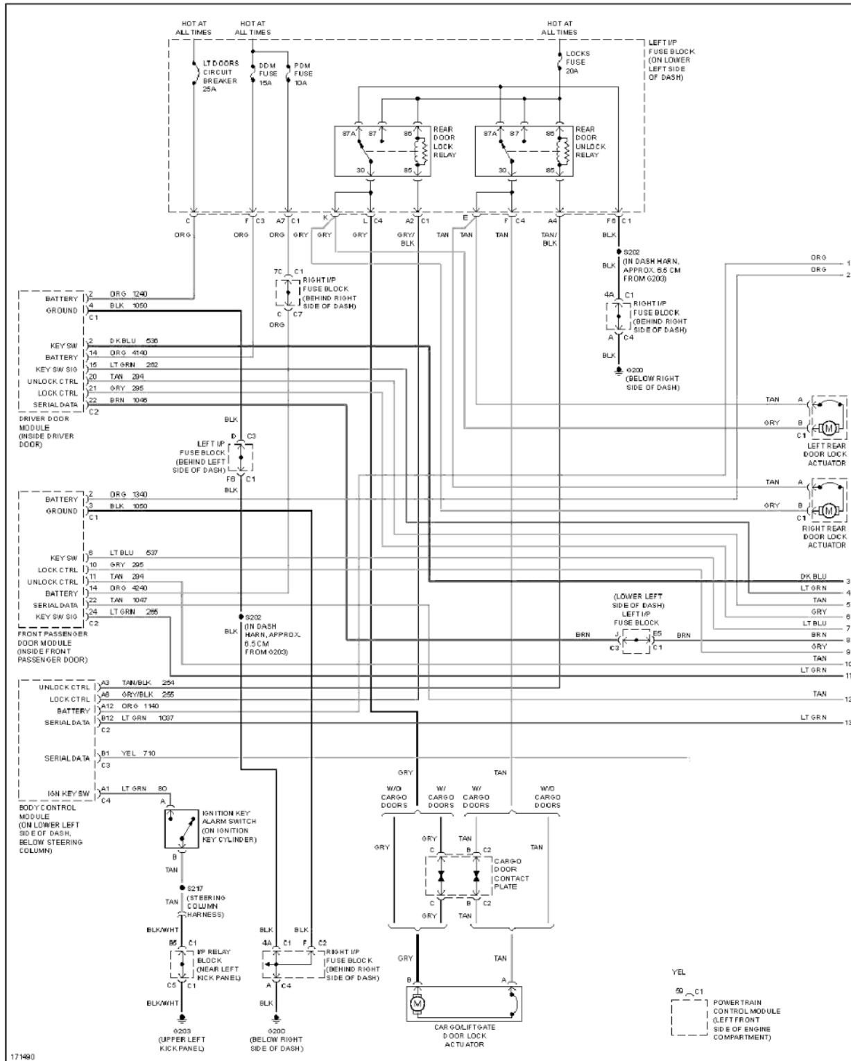
Fig. 72: Power Door Locks Circuit (1 of 2)
